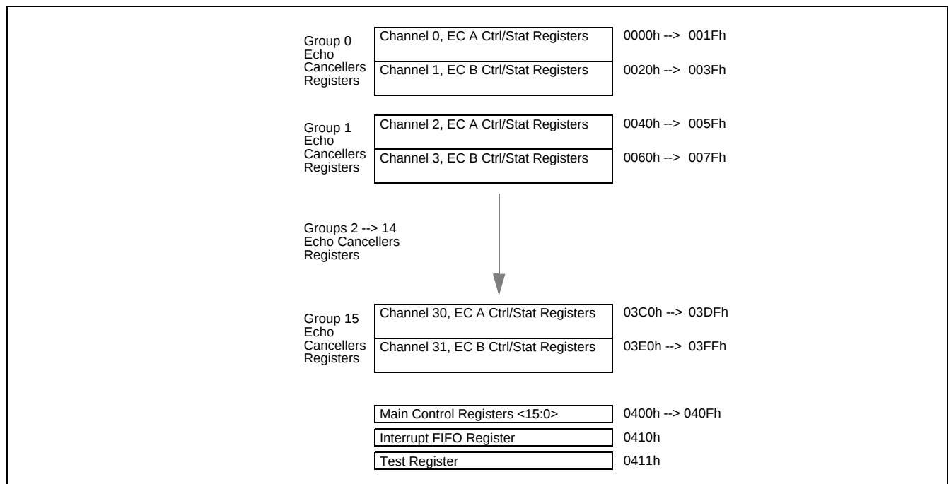
Figure 8 - Memory Mapping
