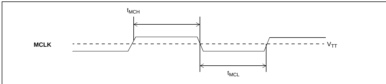
Figure 12 - Master Clock
