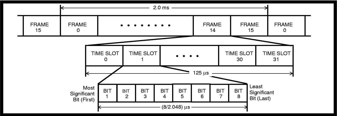
Figure 30 - PCM 30 Format
