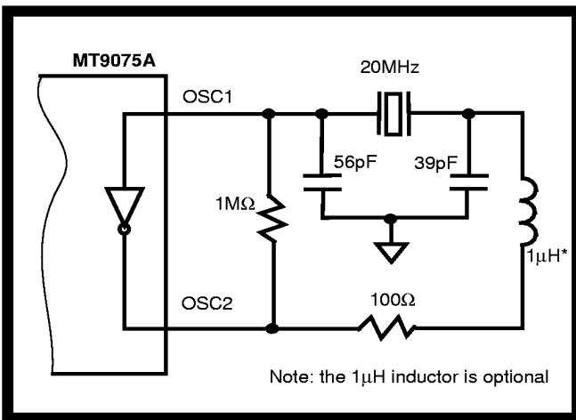
Figure 7 - Crystal Oscillator Circuit
