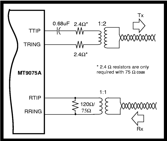
Figure 4 - Analog Line Interface
