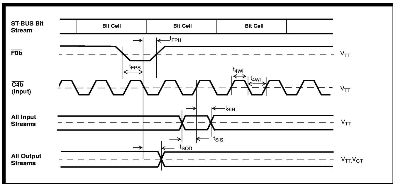
Figure 22 - ST-BUS Timing Diagram
