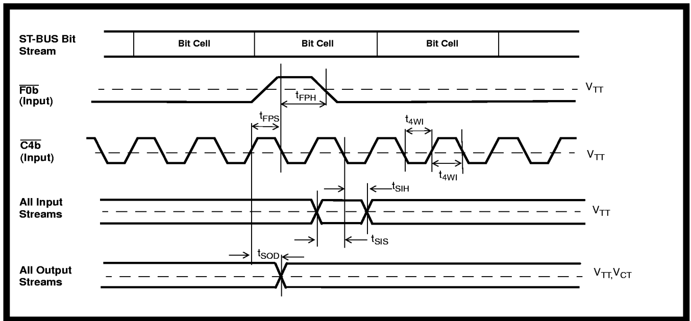
Figure 25 - GCI Timing Diagram (Input Clocks)
