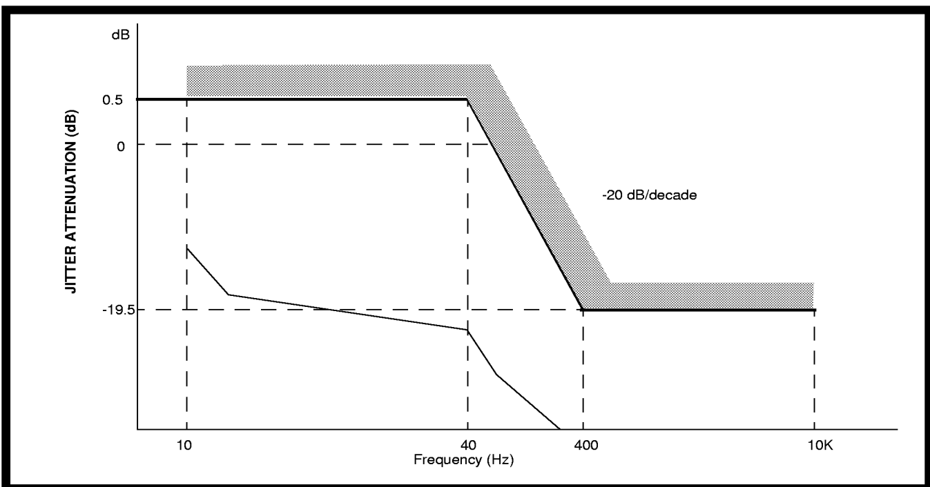
Figure 8 - Typical Jitter Attenuation Curve
