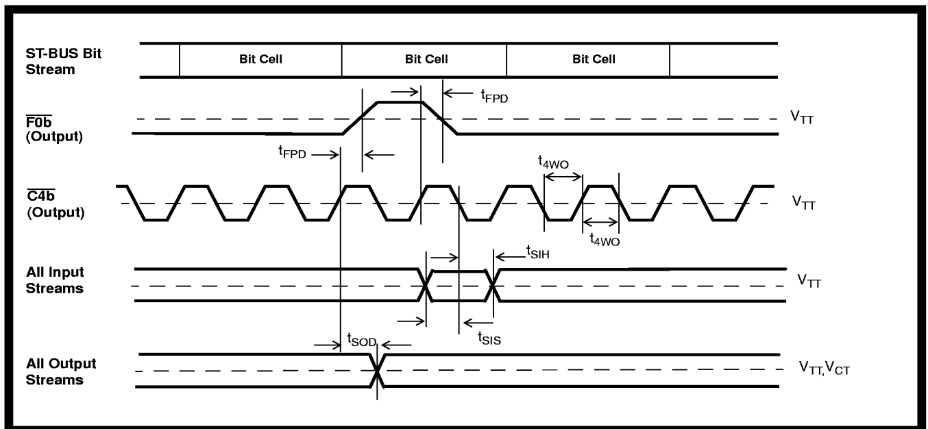
Figure 26 - GCI Timing Diagram (Output Clocks)
