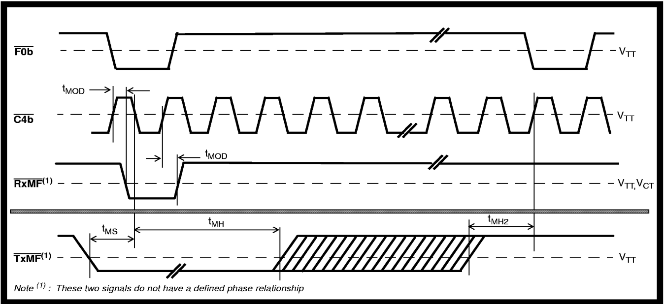
Figure 29 - Multiframe Timing Diagram
