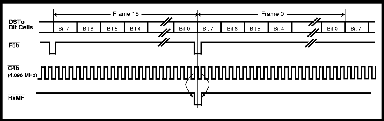
Figure 27 - Receive Multiframe Functional Timing
