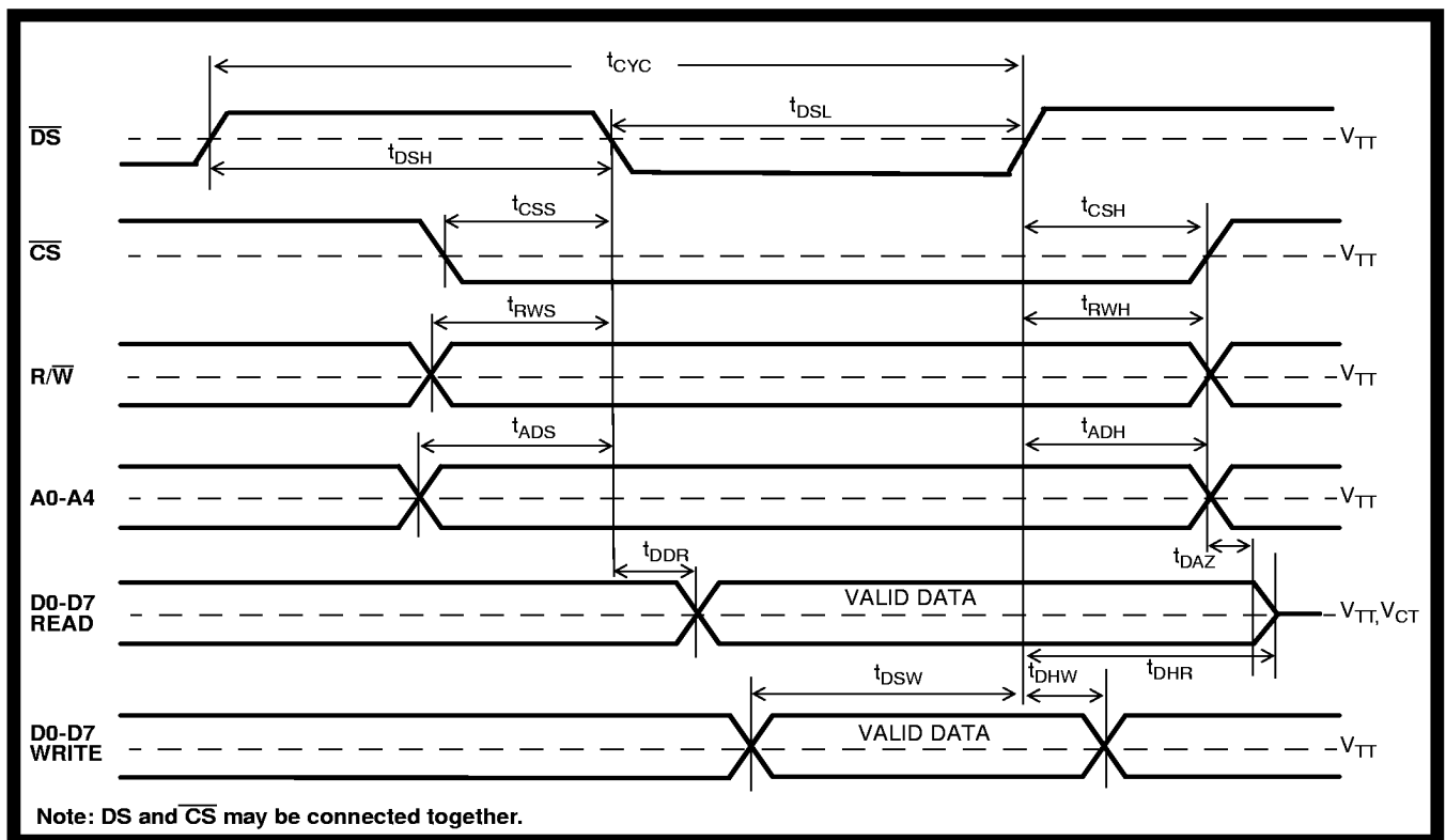
Figure 11 - Motorola Microprocessor Timing
