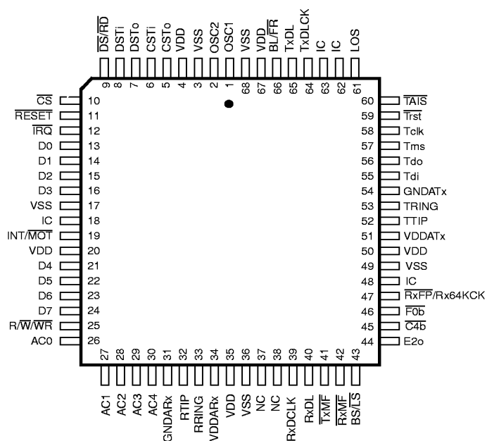
68 PIN PLCC
