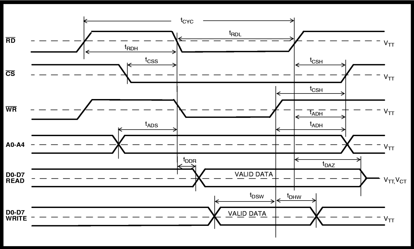
Figure 12 - Intel Microprocessor Timing
