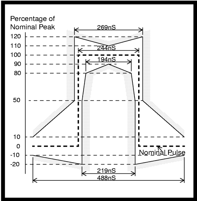
Figure 5 - Pulse Template (G.703)
