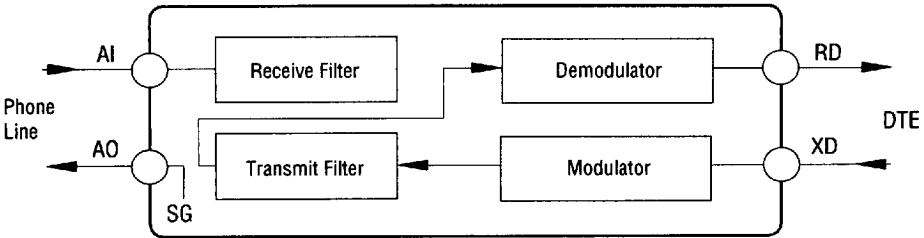
Figure 4 Analog Loop Back Test Mode
