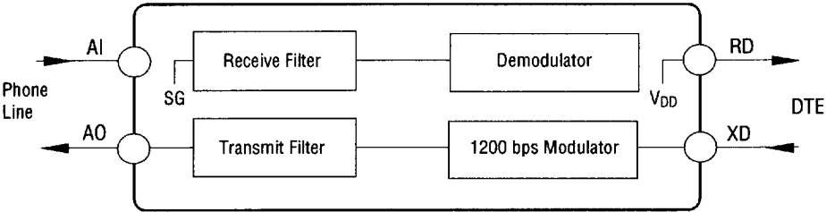
Figure 2 1200 bps Transmit Mode
