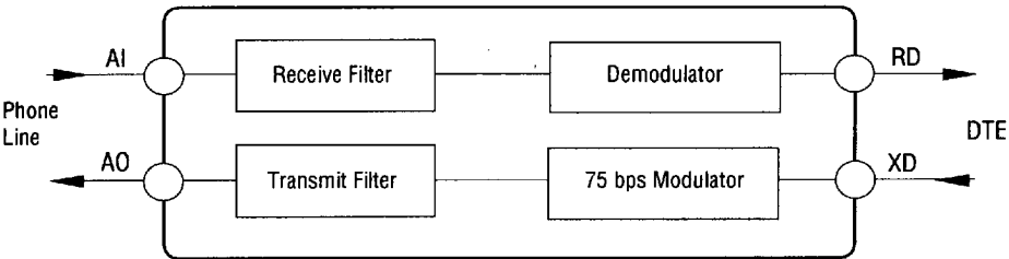
Figure 3 1200 bps Receive & 75 bps Transmit Mode
