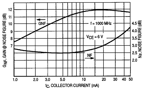
Figure 7. Noise Figure & Gain @ Noise Figure versus Collector Current
