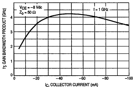
Figure 8. Gain-Bandwidth Product versus Current
