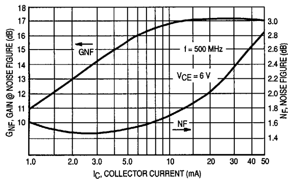
Figure 6. Noise Figure & Gain @ Noise Figure versus Collector Current
