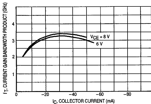
Figure 4. Current Gain Bandwidth Product versus Collector Current
