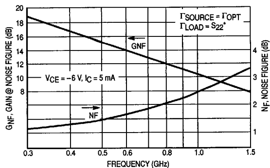
Figure 5. Noise Figure & Gain @ Noise Figure versus Frequency
