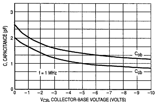
Figure 1. Junction Capacitance versus Voltage
