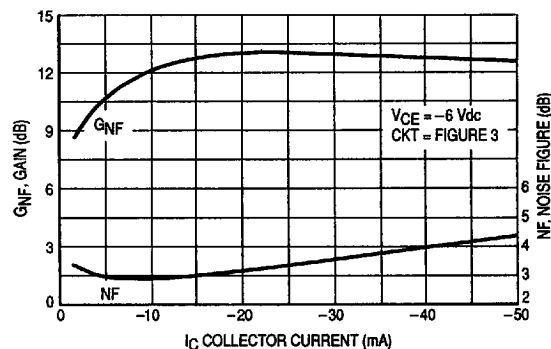
Figure 12. Tuned Circuit — Frequency 1.0 GHz
