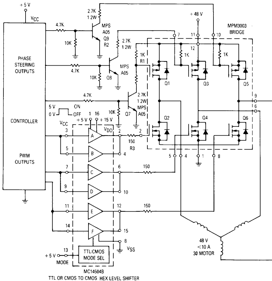
Figure 32. MPM3003 30 Motor Controller
