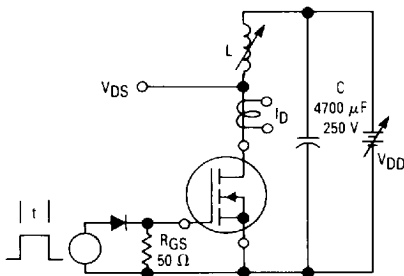
Figure 24. Unclamped Inductive Switching Test Circuit
