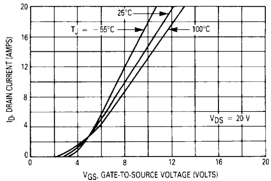
Figure 4. Transfer Characteristics
