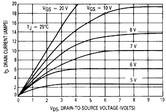
Figure 2. On-Region Characteristics
