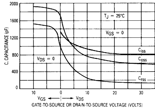
Figure 14. Capacitance Variation
