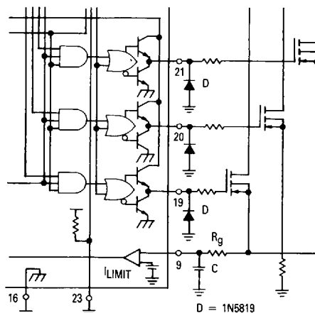
Figure 31. Damping MOSFET Oscillations
