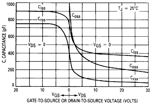
Figure 13. Capacitance Variation
