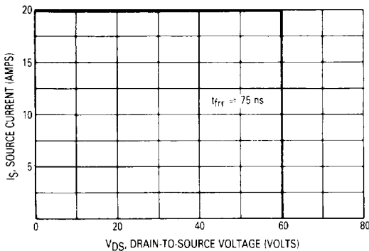
Figure 22. Commutating Safe Operating Area (CSOA)
