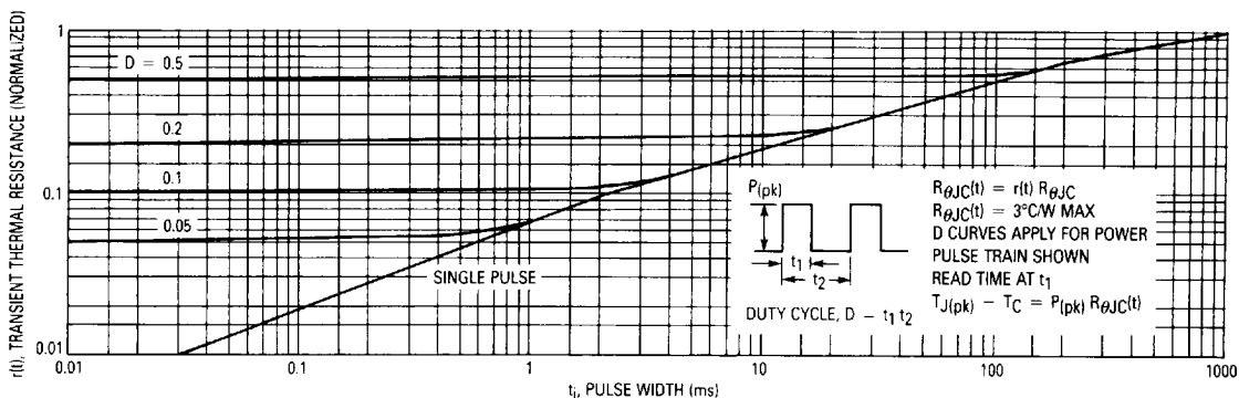
Figure 20. Thermal Response (P-Channel)
