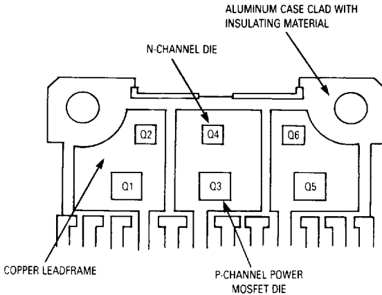
Figure 26. Internal Construction of the MPM3003
