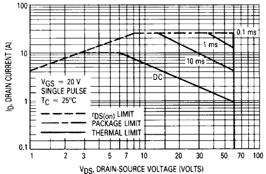
Figure 18. Maximum Rated Forward Biased Safe Operating Area
