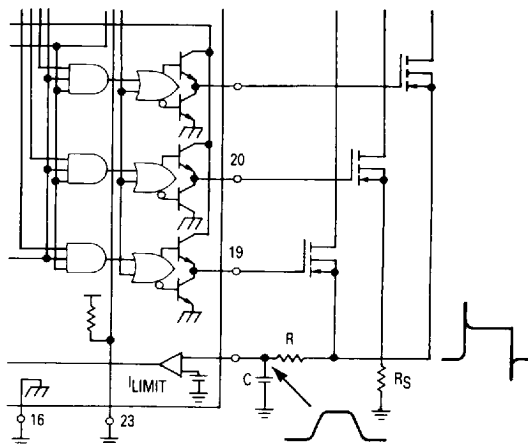
Figure 30. Current Waveform Spike Suppression
