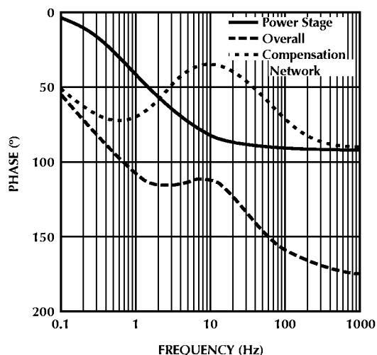
Figure 6. Voltage Loop Phase
