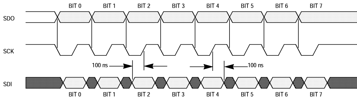
Figure 7-2. SIOF Timing Diagram
