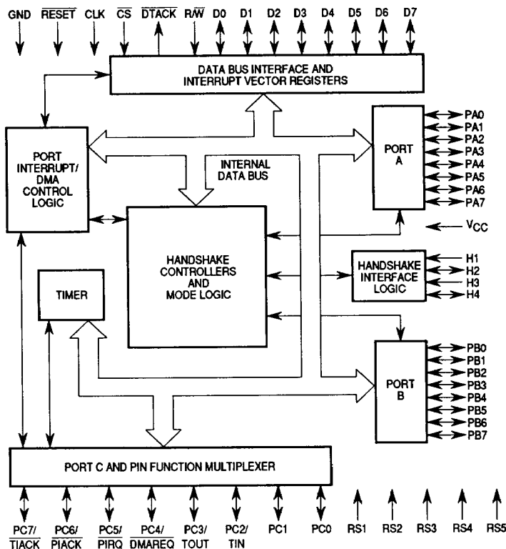
Figure 1. Block Diagram
