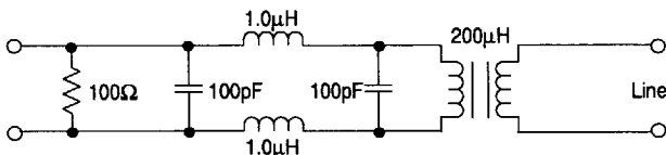
Figure 30. Test Load H
