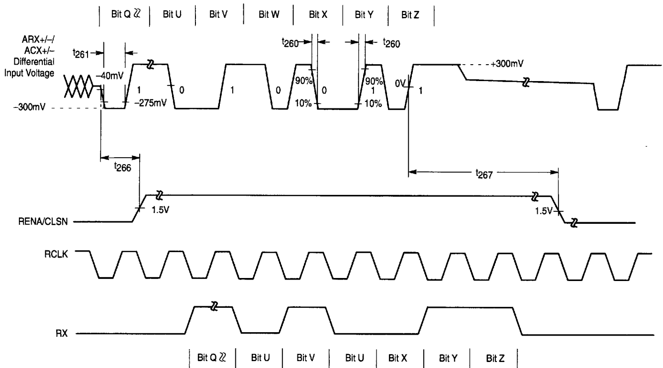
Figure 40. ARX/ACX Timing
