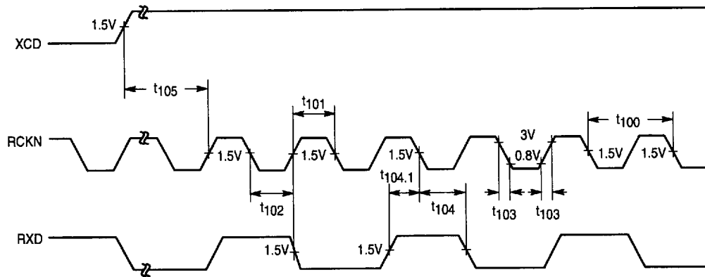
Figure 17. Receive Timing (Fujitsu End of Frame)
