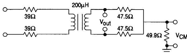
Figure 22. Test Load C
