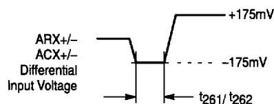
Figure 39. ARX/ACX Timing
