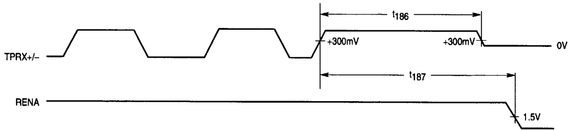
Figure 33. RENA Deassertion Delay from Last Valid Positive Transition of TPRX Pair
