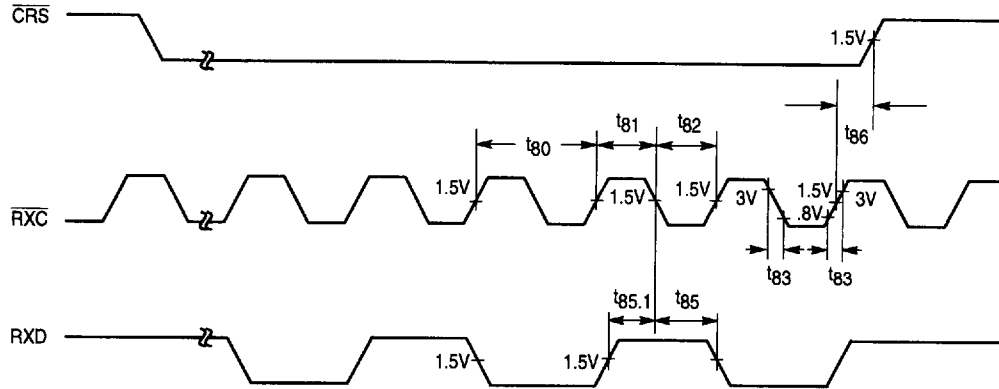
Figure 14. Receive Timing (Intel)
