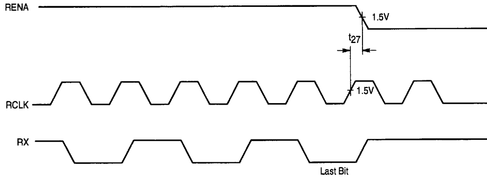
Figure 12. Receive Timing (Motorola End of Frame)
