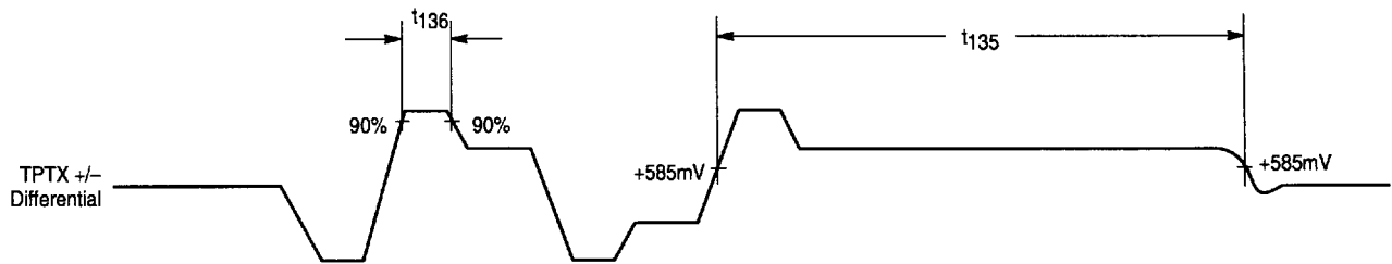
Figure 25. TPTX Transmit Timing (End of Frame) Switching
