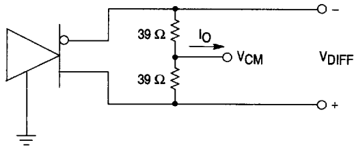
Figure 6. AUI Common Mode Termination
