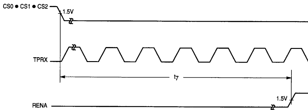
Figure 9. Receive Phase-Locked-Loop Switching
