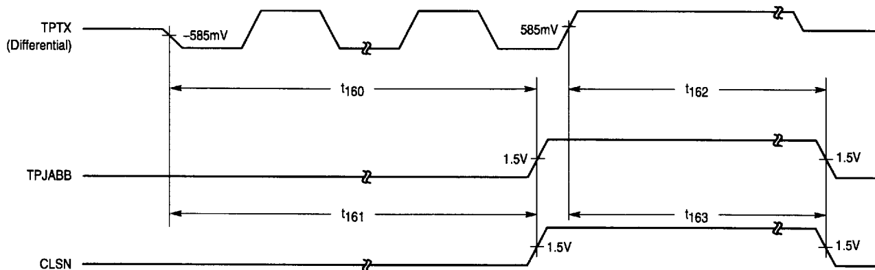
Figure 28. TPJABB Switching
