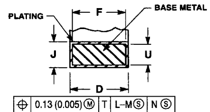
SECTION AB-AB ROTATED 90° CLOCKWISE
