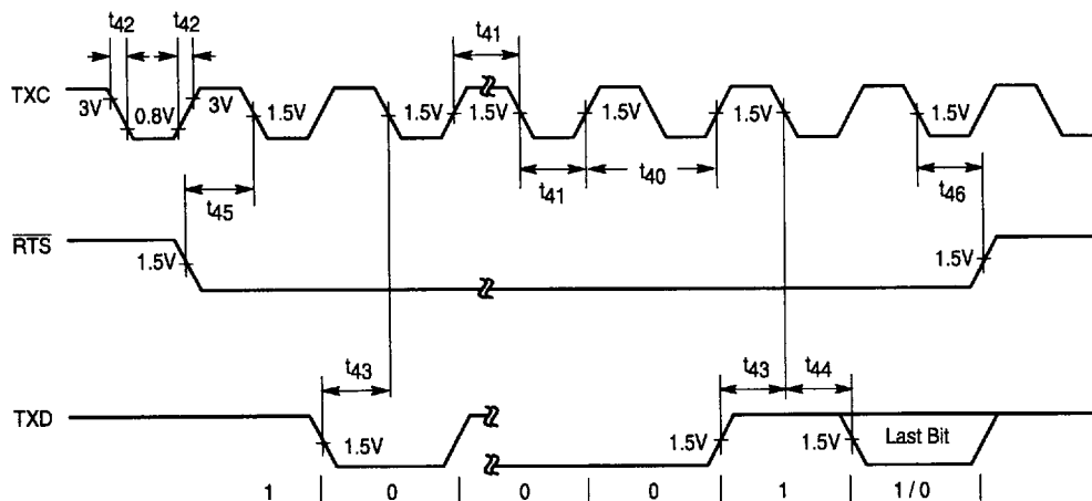
Figure 13. Transmit Timing (Intel)
