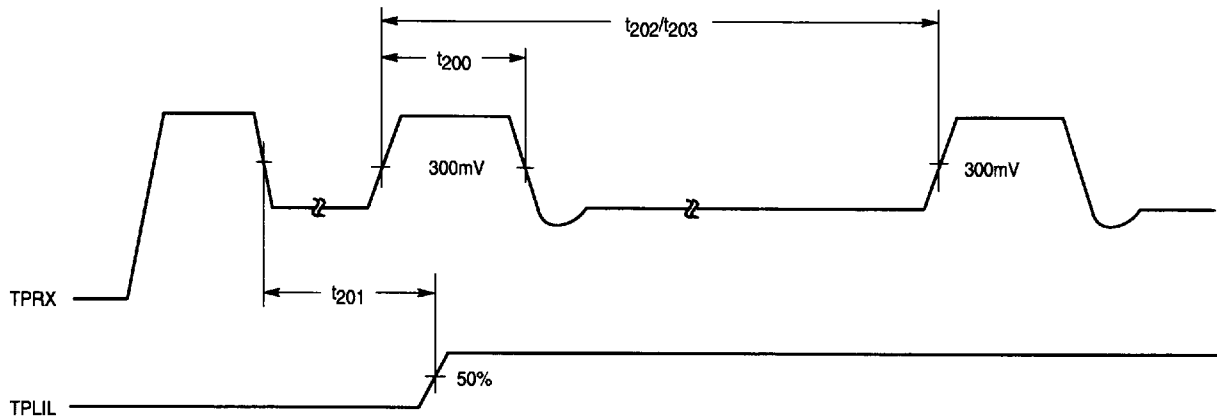
Figure 34. TP Receive Link Integrity Switching
