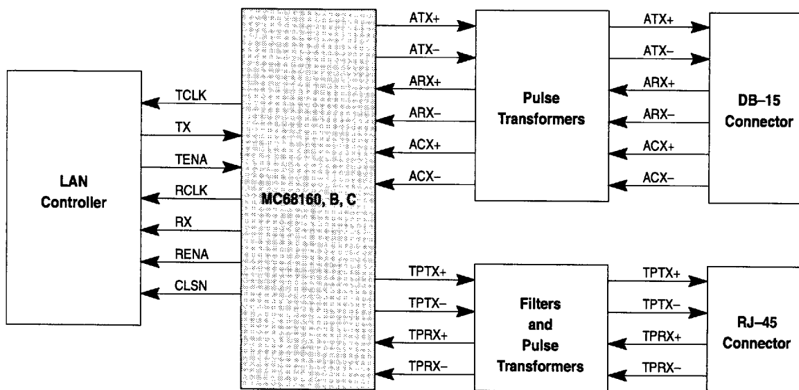
Figure 2. Applications Block Diagram
