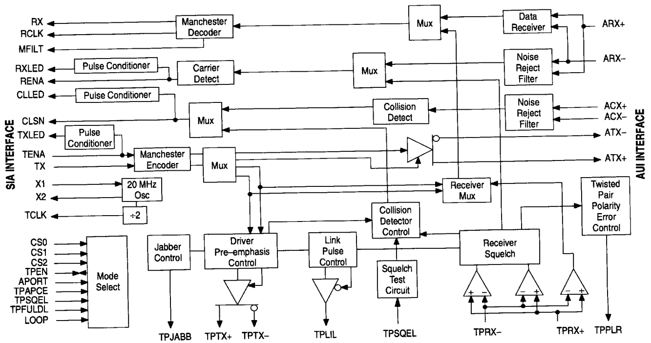
Figure 1. 10Base-T Interface Block Diagram
