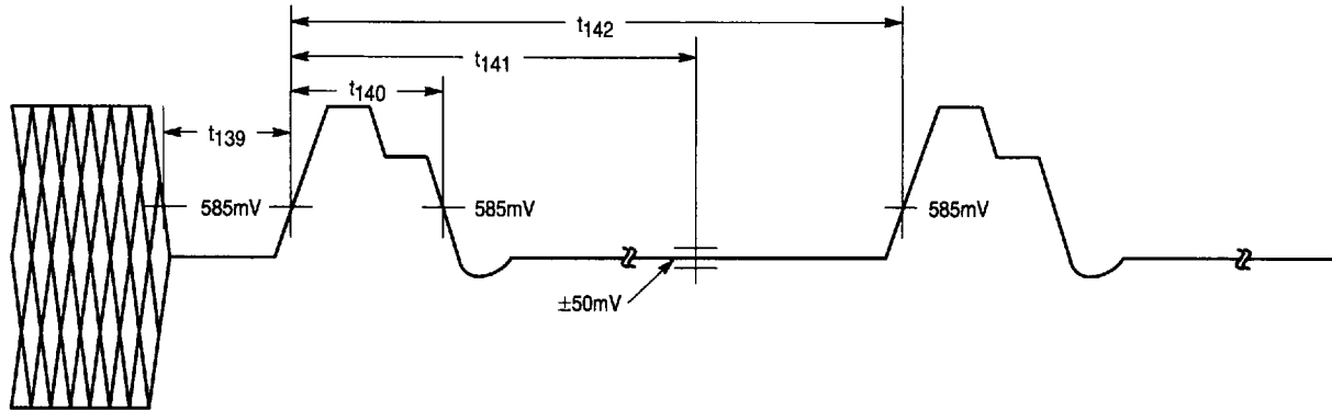
Figure 27. TPTX+/- Link Pulse Timing
