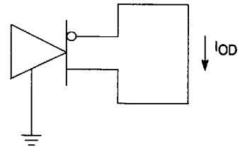
Figure 7. AUI Differential Output Short Circuit Current
