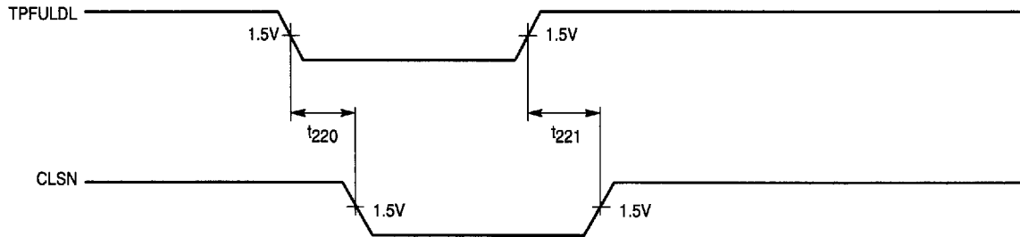
Figure 36. TPTX Full Duplex Timing
