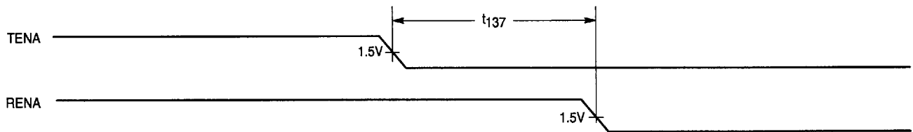
Figure 26. RENA Deassert Delay from TENA
