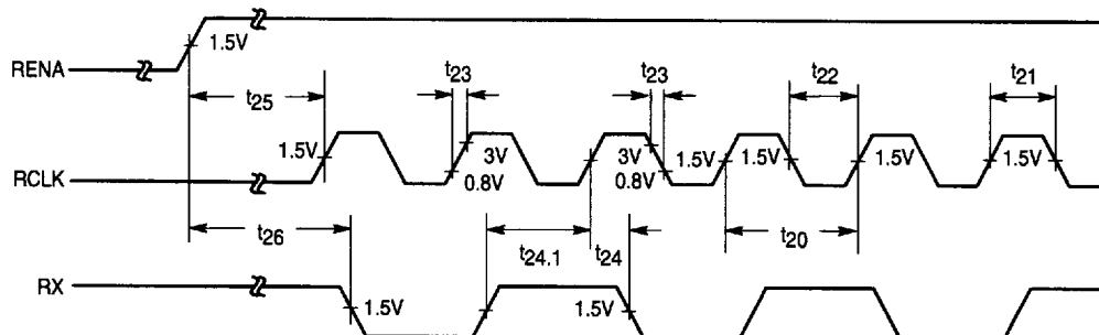
Figure 11. Receive Timing (Motorola Start of Frame)
