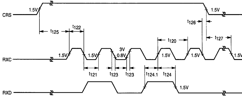
Figure 19. Receive Timing (National)
