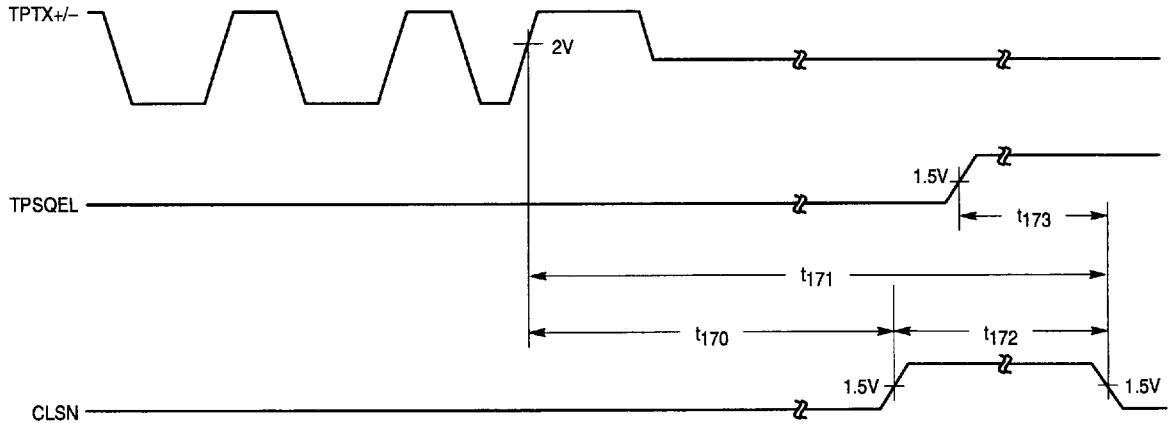
Figure 29. TPTX SQE (CLSN) Timing (End of Frame)
