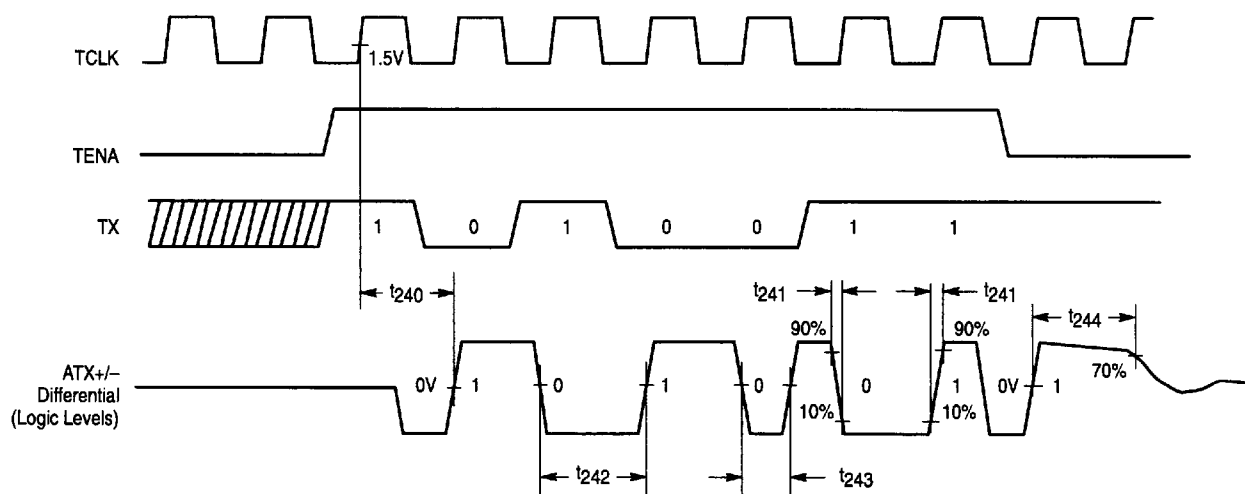
Figure 38. ATX Transmit Timings
