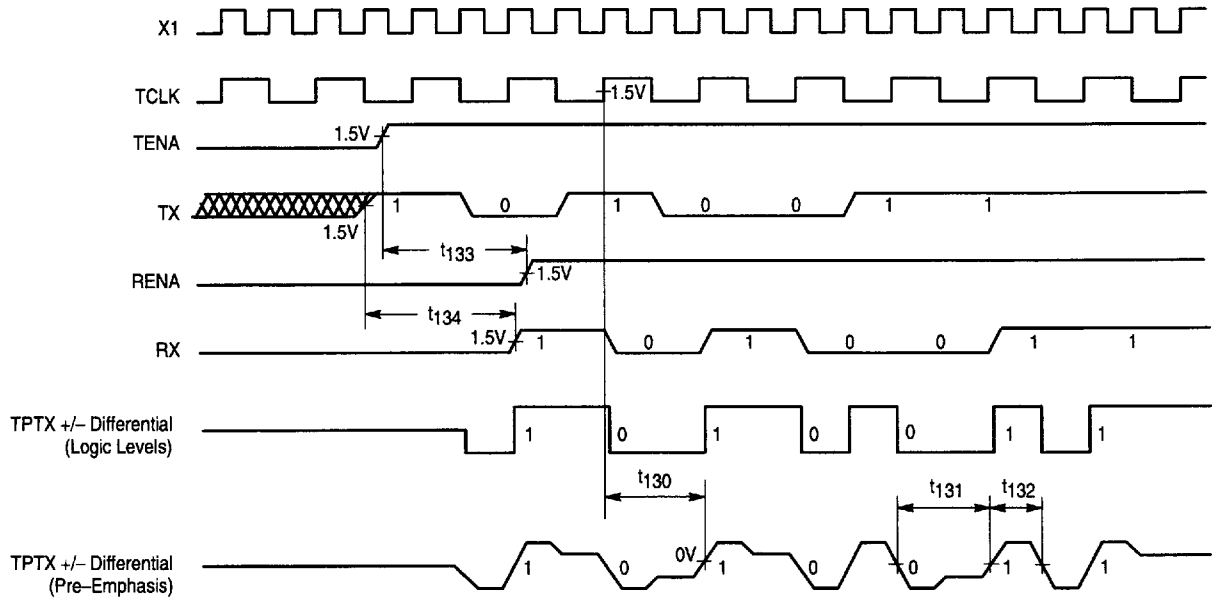
Figure 24. TPTX Transmit Timing (Start of Frame) Switching
