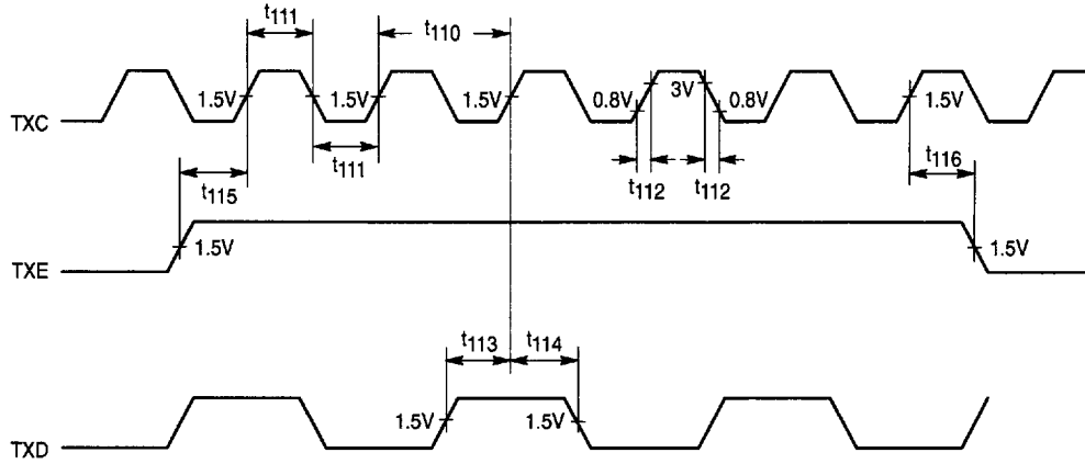
Figure 18. Transmit Timing (National)
