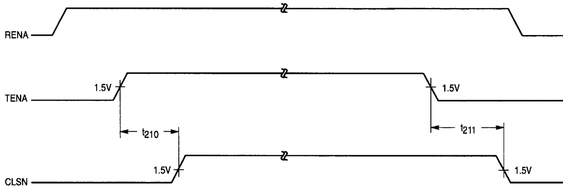
Figure 35. TPTX Collision Timing
