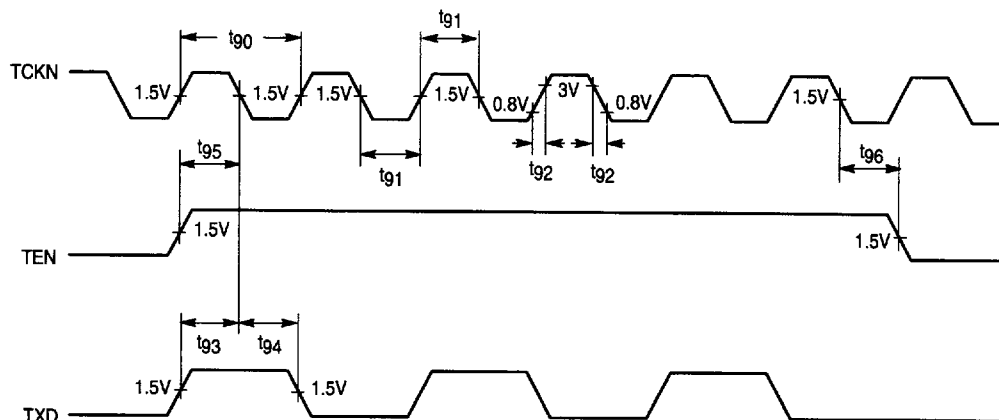
Figure 15. Transmit Timing (Fujitsu)
