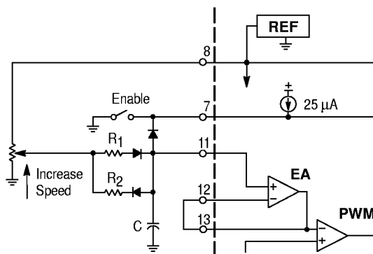
Figure 32. Controlled Acceleration/Deceleration
