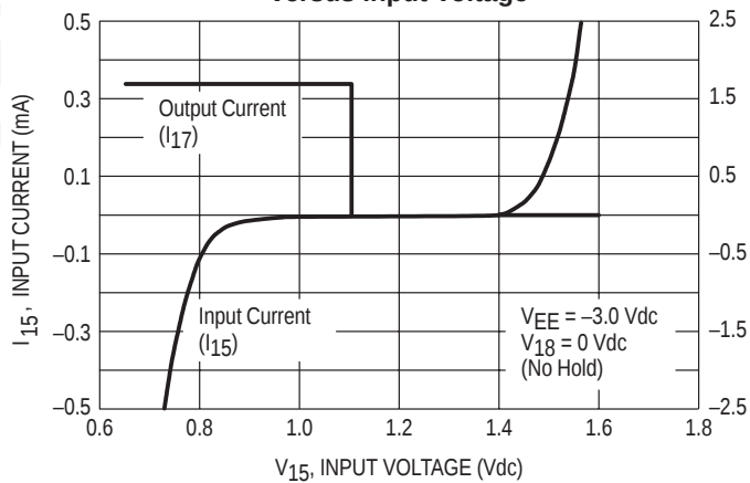
Figure 15. Data Slicer Input/Output Currents versus Input Voltage
