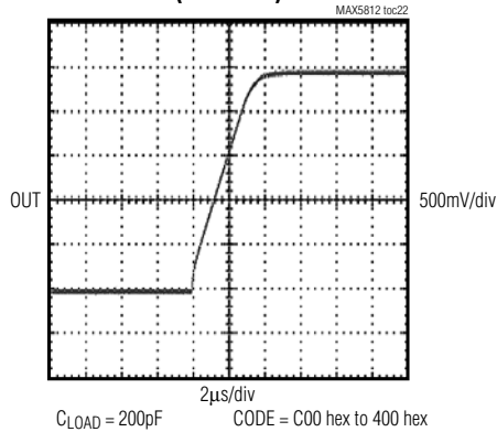
SETTLING TIME (NEGATIVE)
