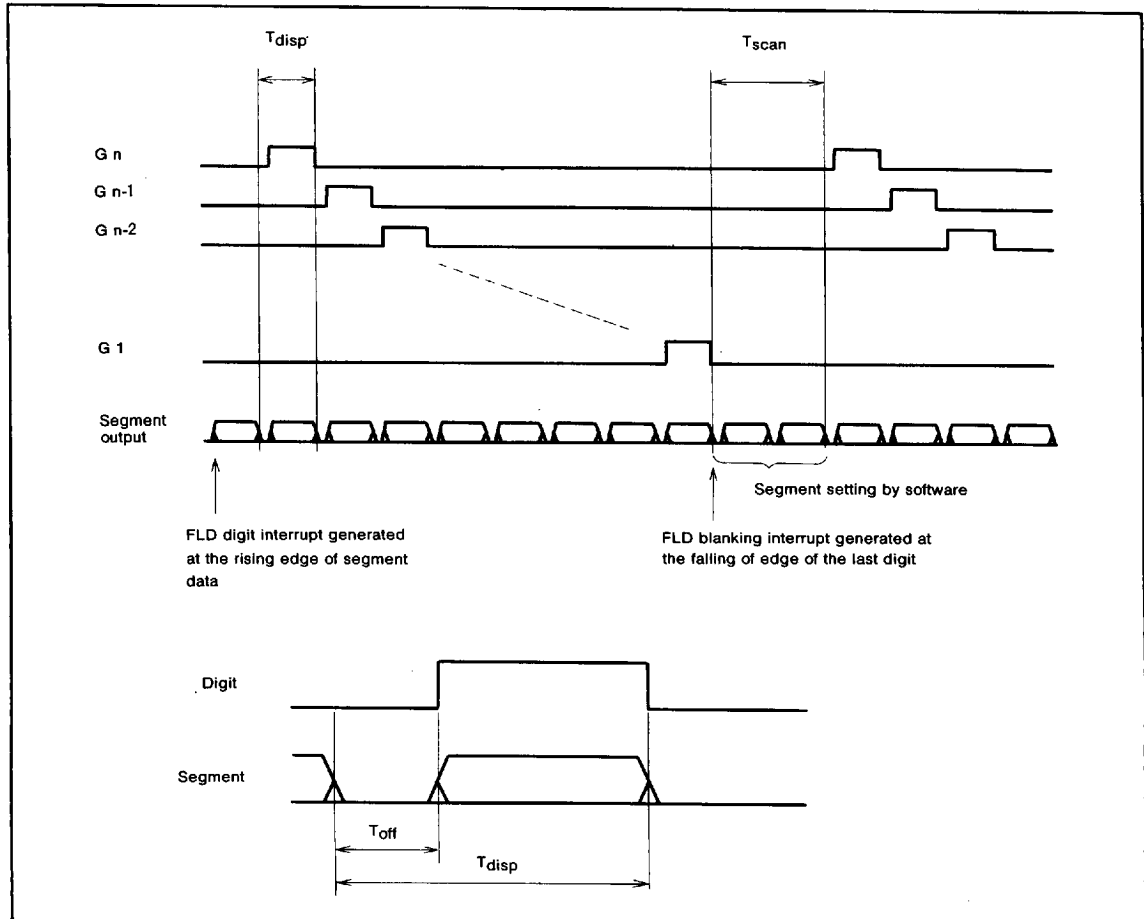
Fig. 33 FLDC timing
