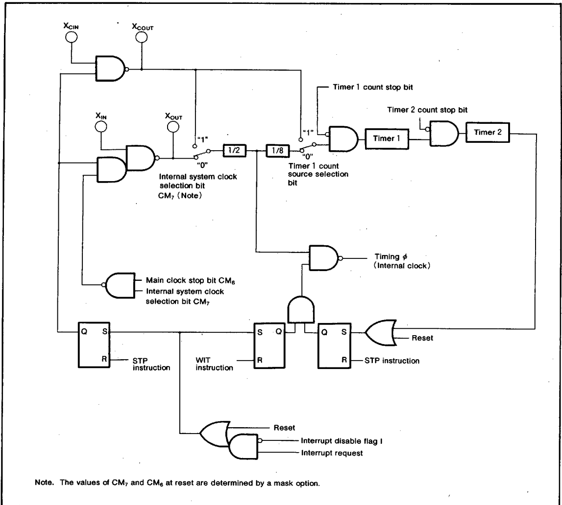
Fig. 40 System clock generation circuit block diagram
