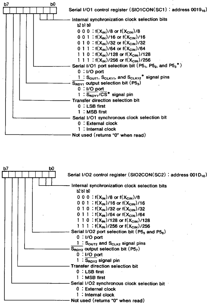
Fig. 12 Structure of serial I/O control registers
