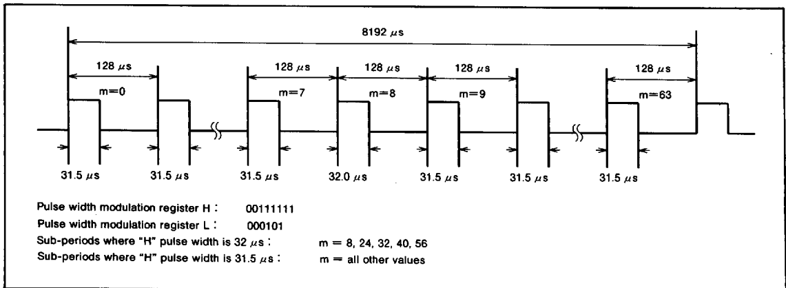
Fig. 22 PWM timing
