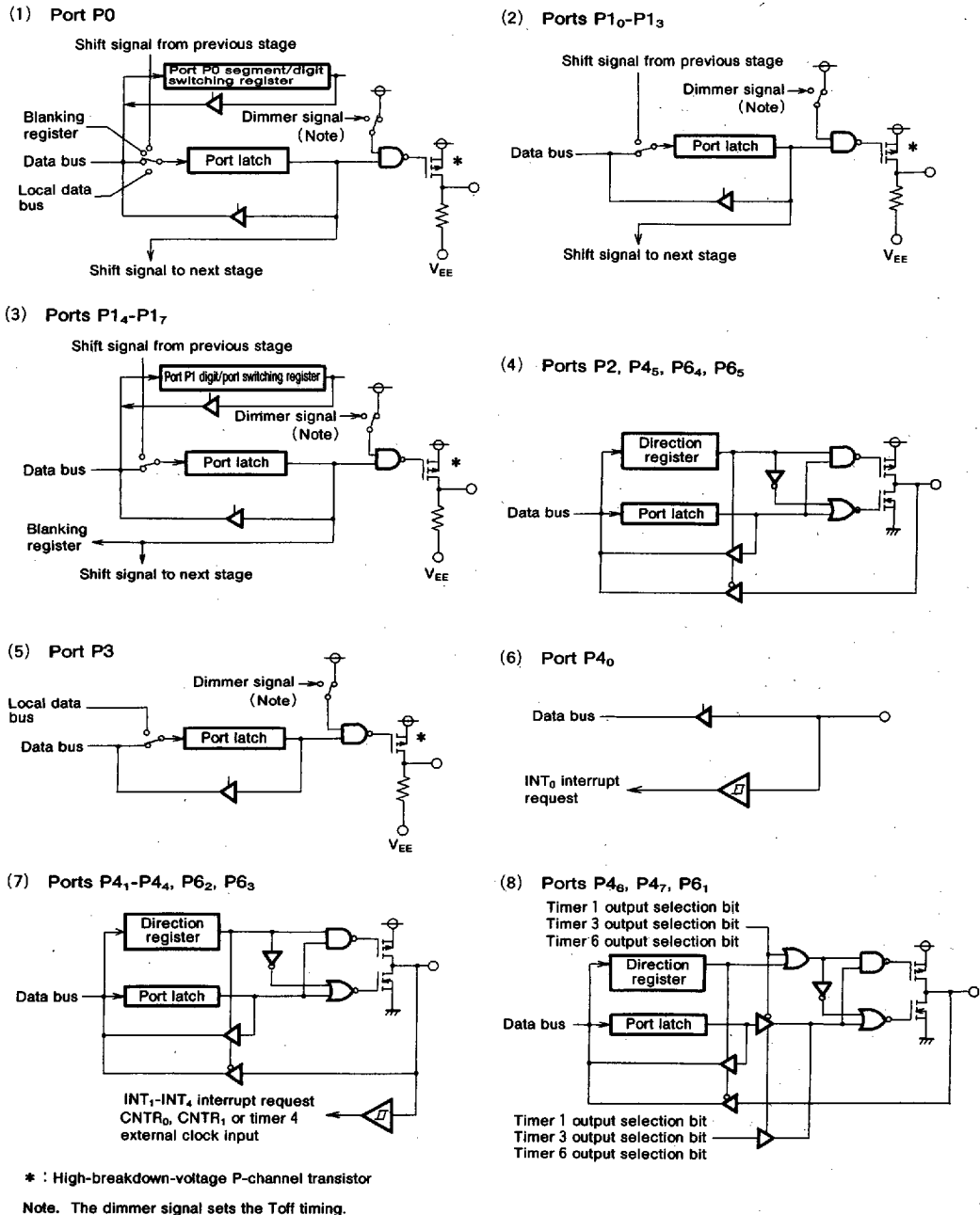
Fig. 4 Port block diagram (1)
