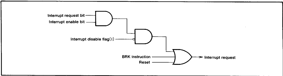
Fig. 6 Interrupt control
