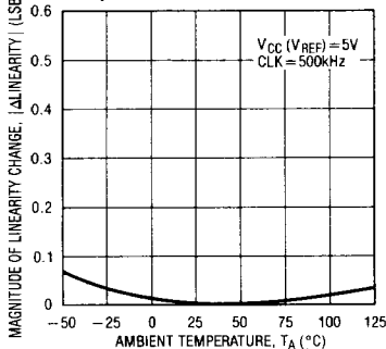
Change in Linearity Error vs Temperature
