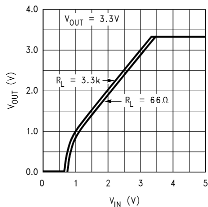
Dropout Characteristics
