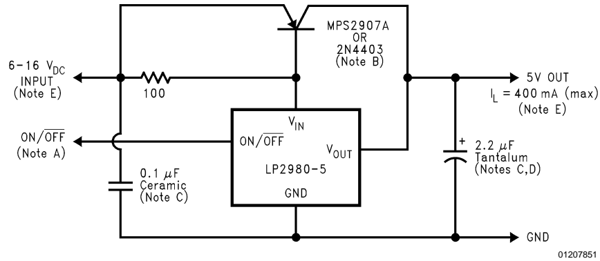
FIGURE 5. 5V/400mA Regulator
