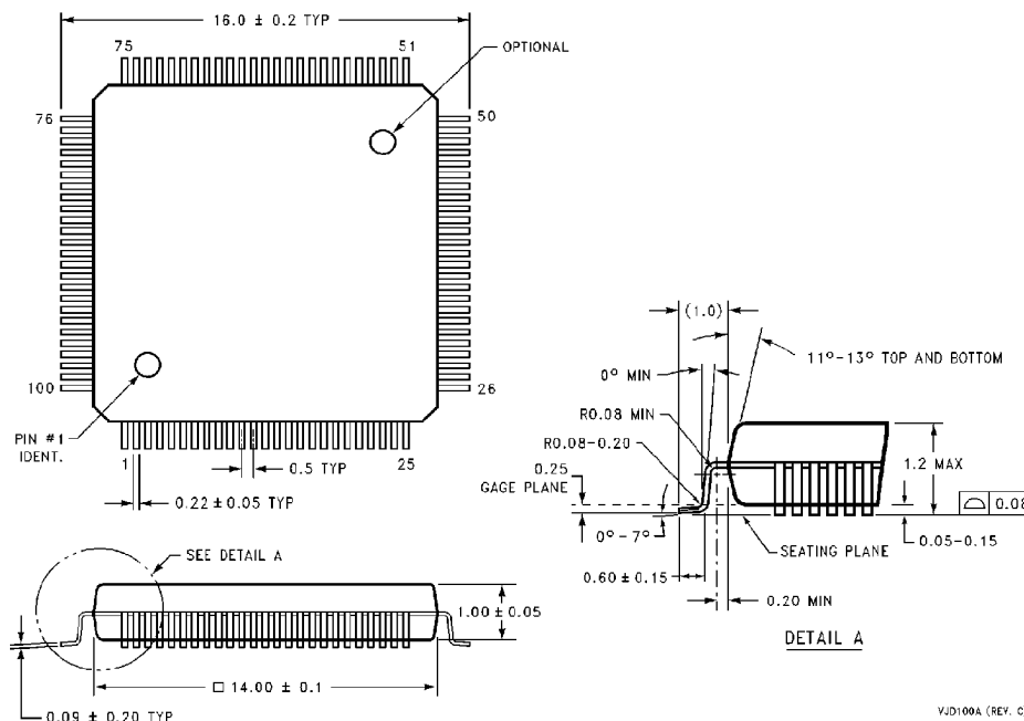
100-Pin Thin Plastic Quad FlatPac (JEDEC) (TQFP) NS Package Number VJD100A Order Number LM9831VJD
