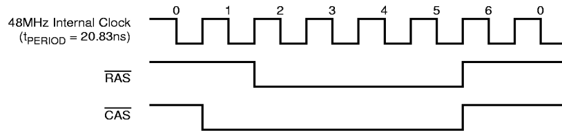
Figure 2: DRAM Refresh ( \overline{\text{CAS}} before \overline{\text{RAS}} )
