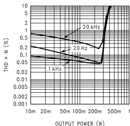
THD+N vs Output Power at V_{DD} = 3V , 8\Omega R_L
