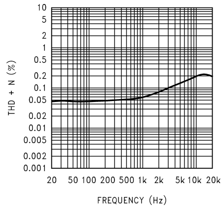
THD+N vs Frequency V_{DD} = 3V , 8\Omega R_L , and PWR = 250mW
