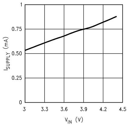
Supply Current at No Load
