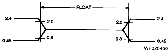
Float Waveform
