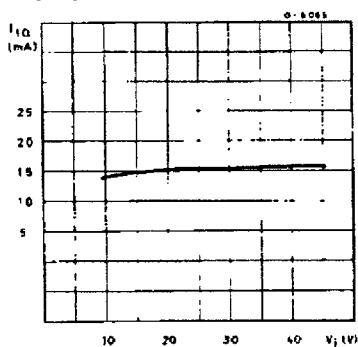
Figure 4. Quiescent drain current vs. supply voltage (0% duty cycle)
