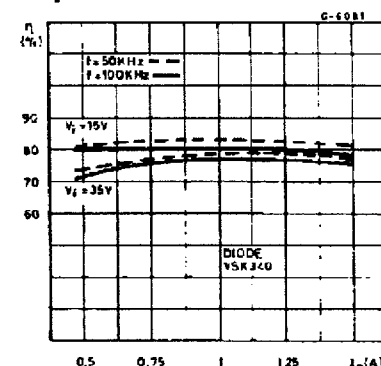
Figure 21. Efficiency vs. output current
