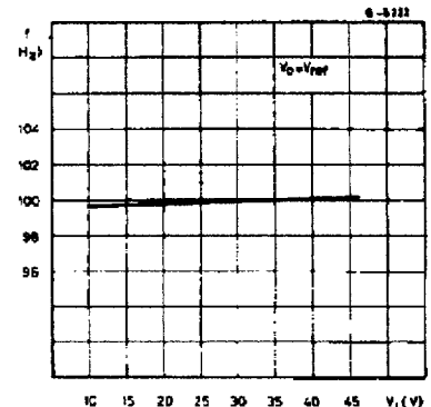
Figure 11. Switching frequency vs. input voltage
