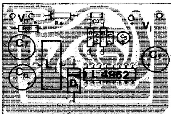
Figure 26. P.C. board and component layout of the circuit of Fig. 25 (1 : 1 scale)
