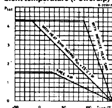
Figure 24. Maximum allowable power dissipation vs. ambient temperature (Powerdip)
