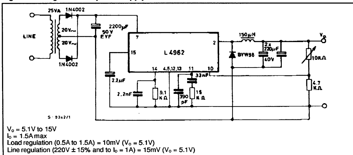
Figure 28. Programmable power supply
