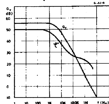
Figure 10. Open loop frequency and phase response of error amplifier
