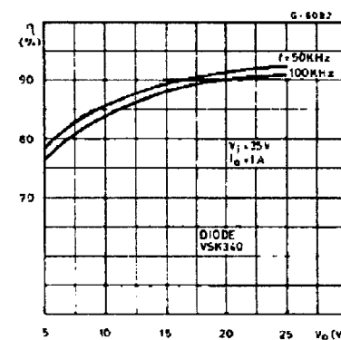
Figure 22. Efficiency vs. output voltage
