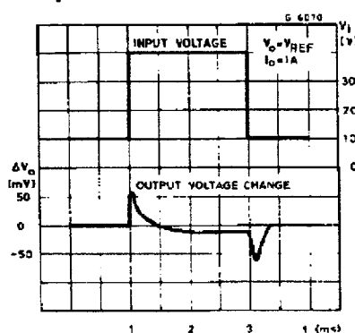
Figure 14. Line transient response
