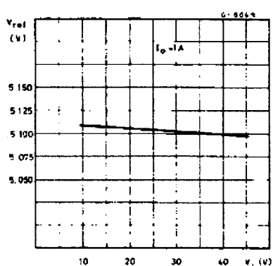
Figure 8. Reference voltage (pin 10) vs. V_I rdip) vs. V_I
