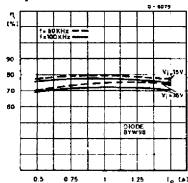
Figure 19. Efficiency vs. output current
