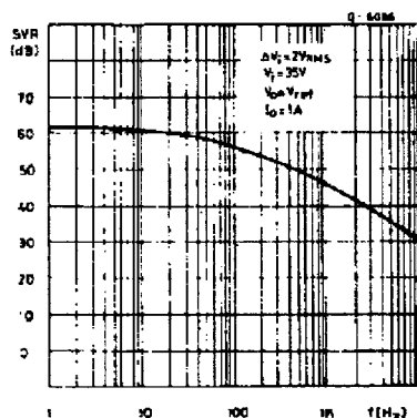
Figure 16. Supply voltage ripple rejection vs. frequency
