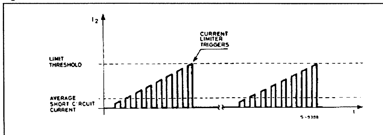
Figure 2. Current limiter waveforms
