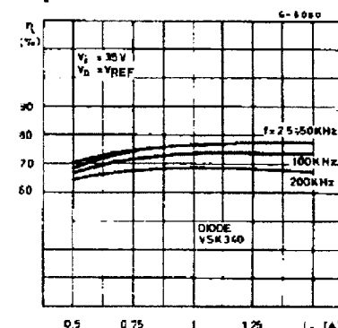
Figure 20. Efficiency vs. output current
