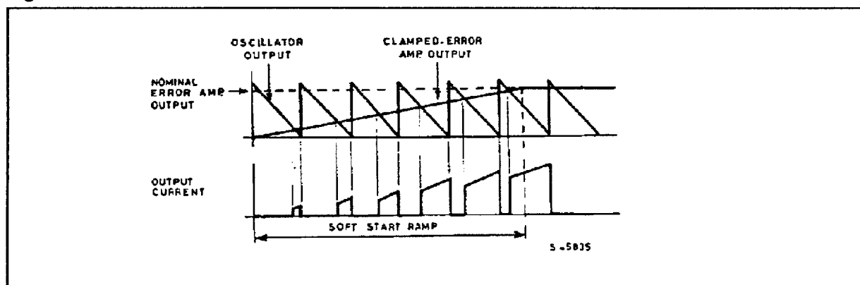
Figure 1. Soft start waveforms
