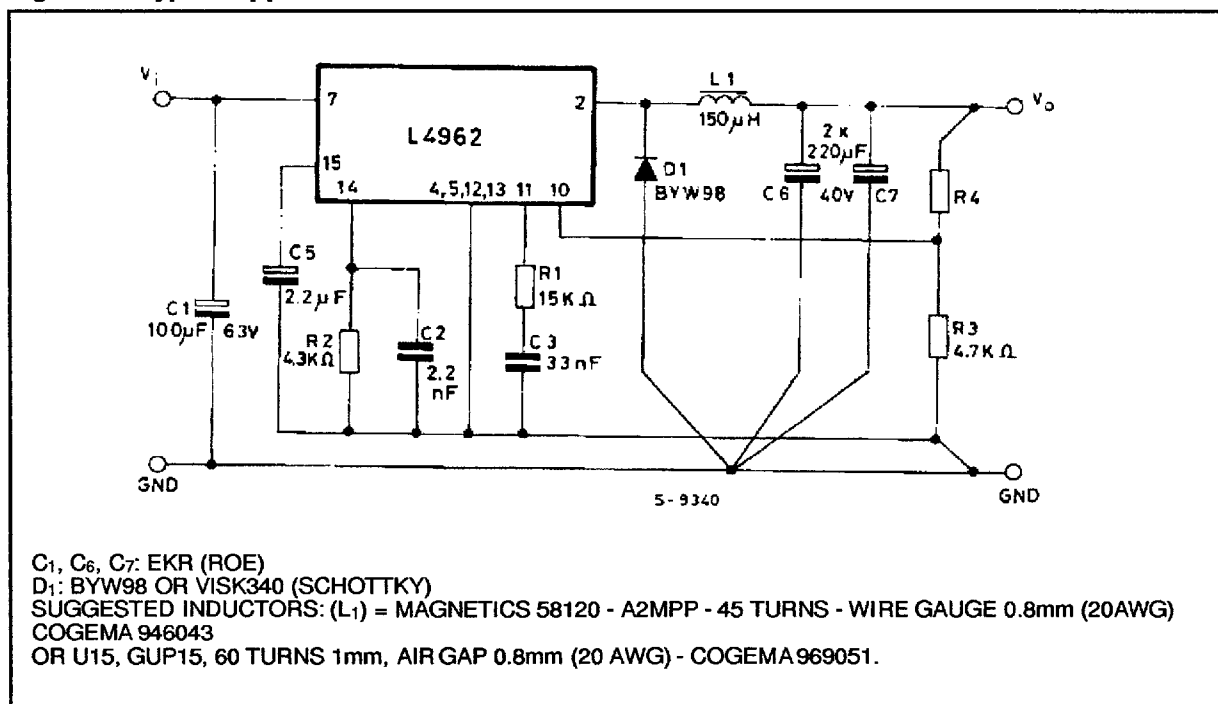
Figure 25. Typical application circuit
