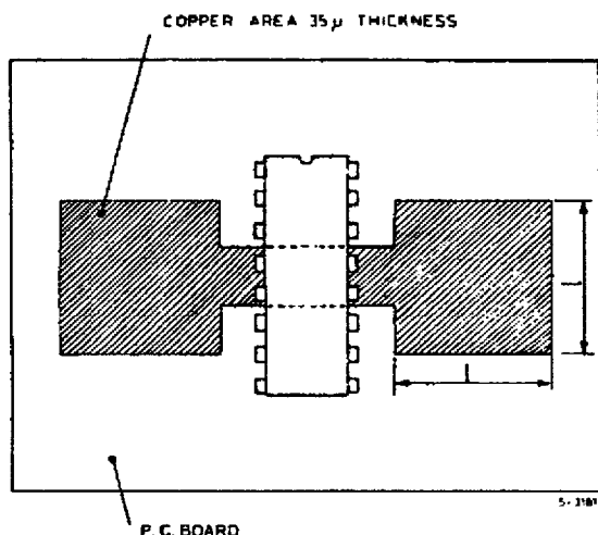
Figure 32. Example of P.C. board copper area which is used as heatsink
