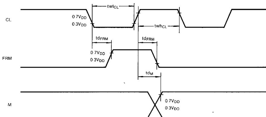
Fig 2. Display control signal waveform
