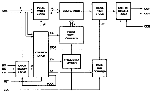
FUNCTIONAL IXDP610 BLOCK DIAGRAM
