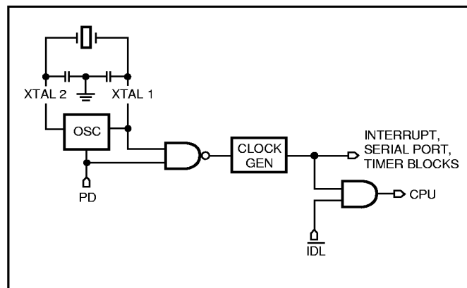
Figure 23. Idle and Power-Down Hardware
