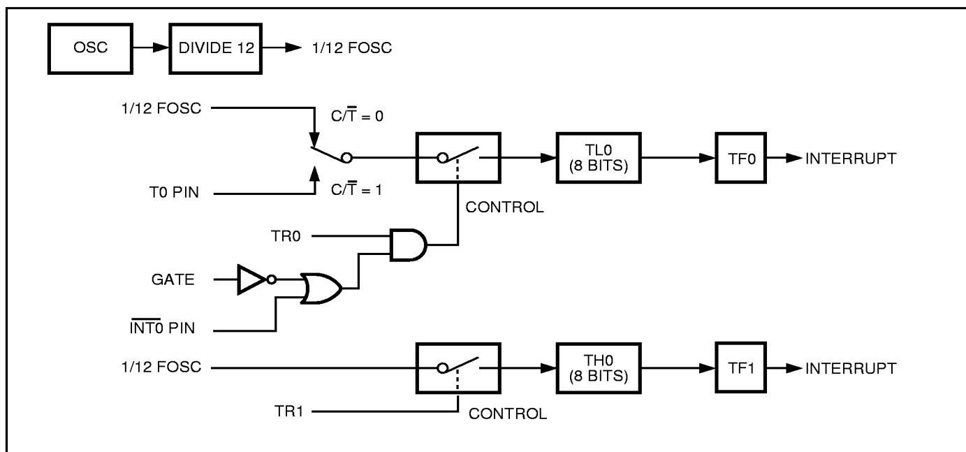
Figure 11. Timer/Counter 0 Mode 3: Two 8-Bit Counters
