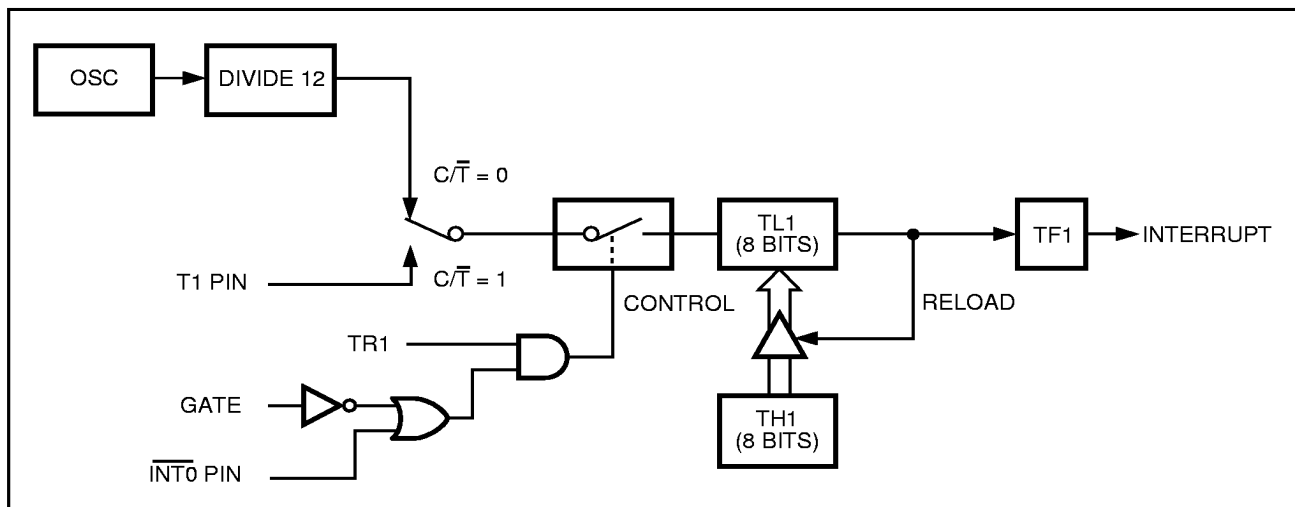
Figure 10. Timer/Counter 1 Mode 2: 8-Bit Auto-Reload
