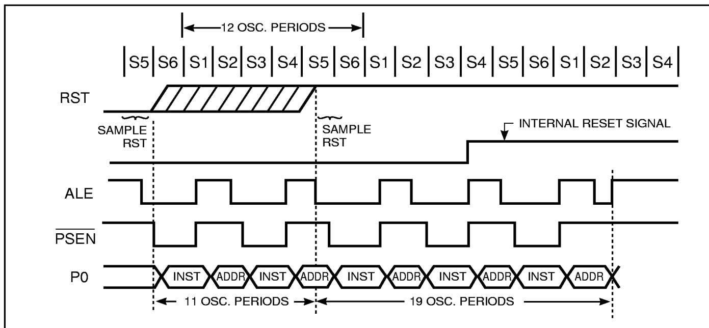
Figure 21. Reset Timing
