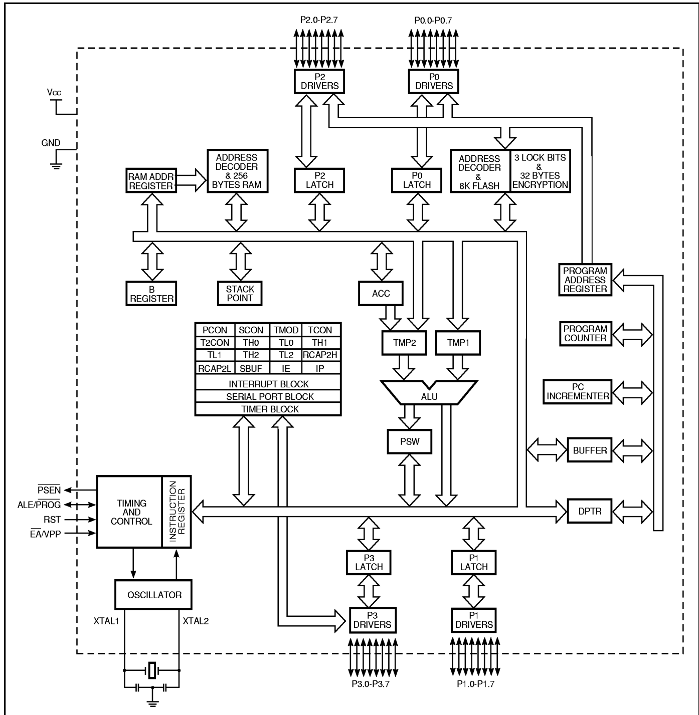
Figure 4. IS89C52 Block Diagram
