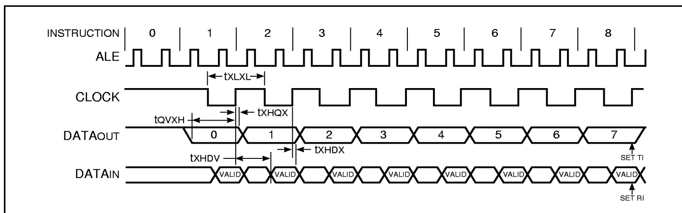
Figure 38. Shift Register Mode Timing Waveform
