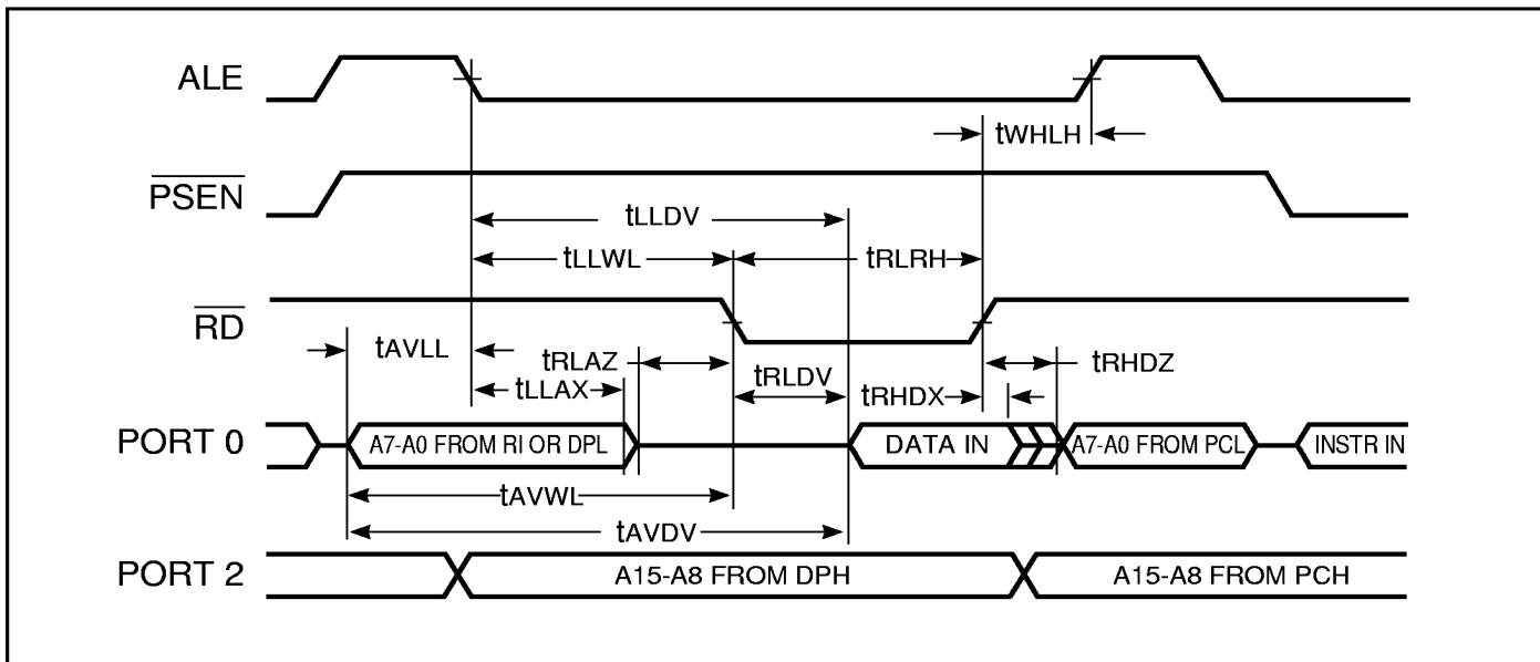
Figure 36. External Data Memory Read Cycle
