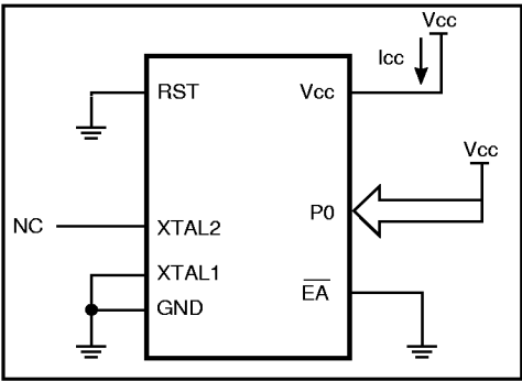
Figure 33. Power-down Mode
