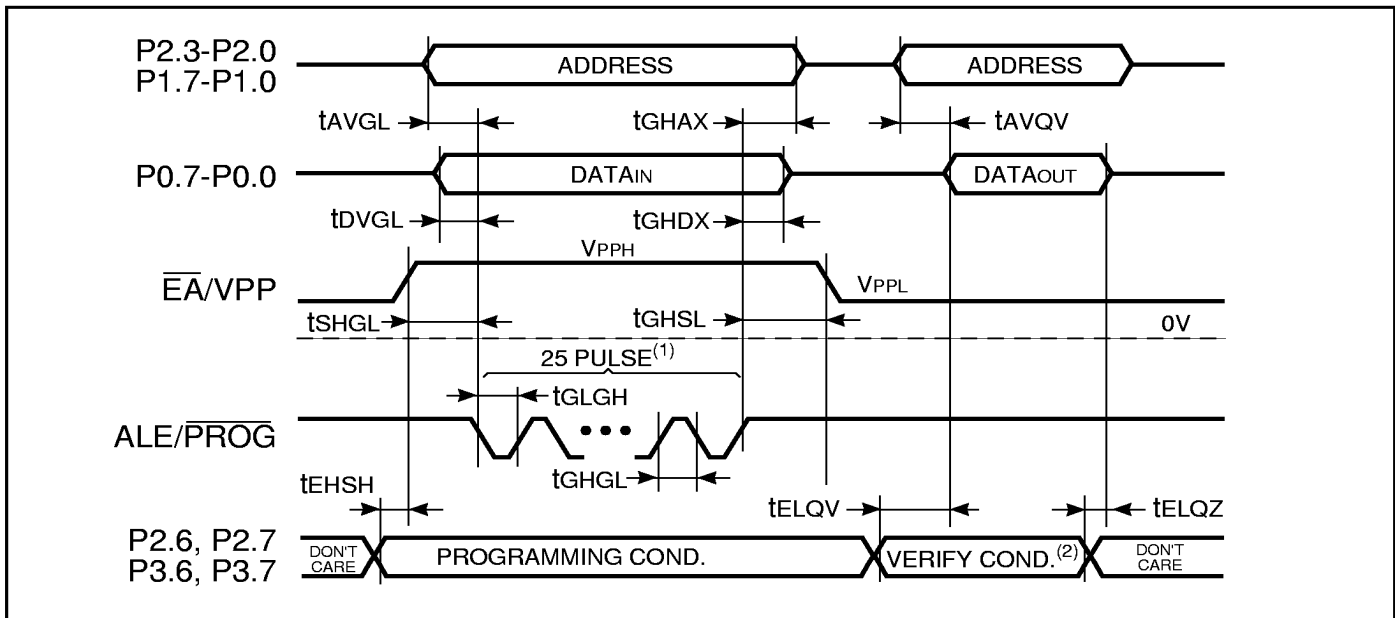
Figure 29. Flash Memory Programming and Verification Timing Waveform
