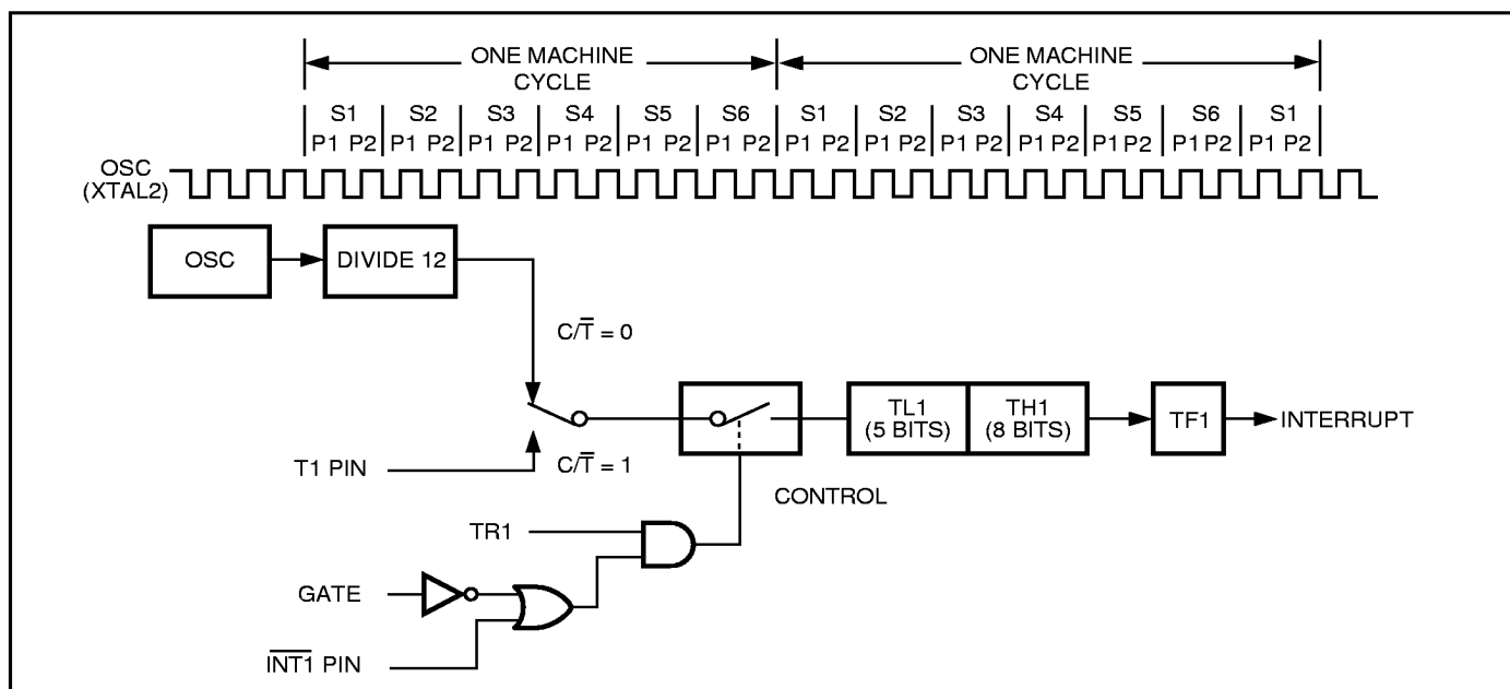
Figure 8. Timer/Counter 1 Mode 0: 13-Bit Counter
