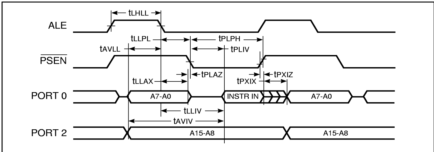
Figure 35. External Program Memory Read Cycle
