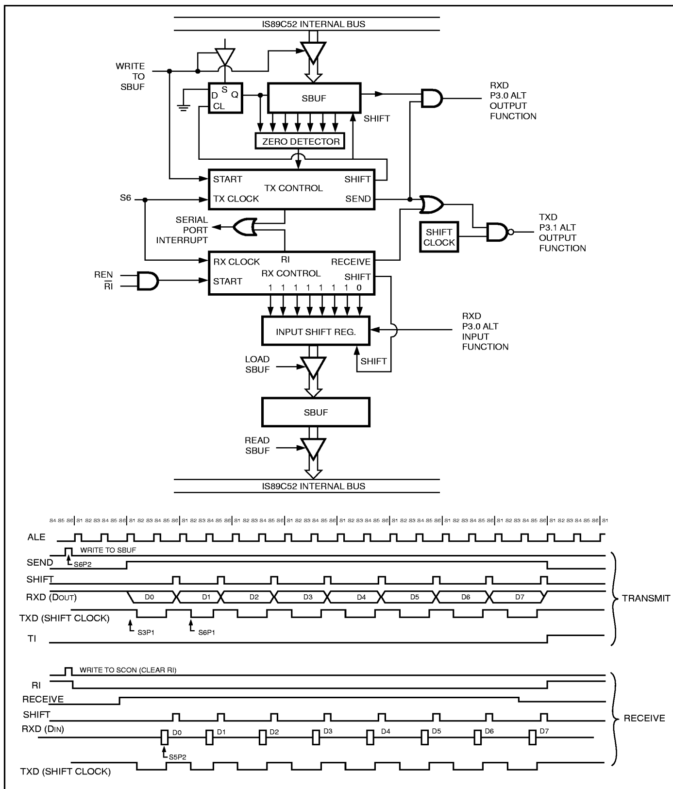
Figure 15. Serial Port Mode 0
