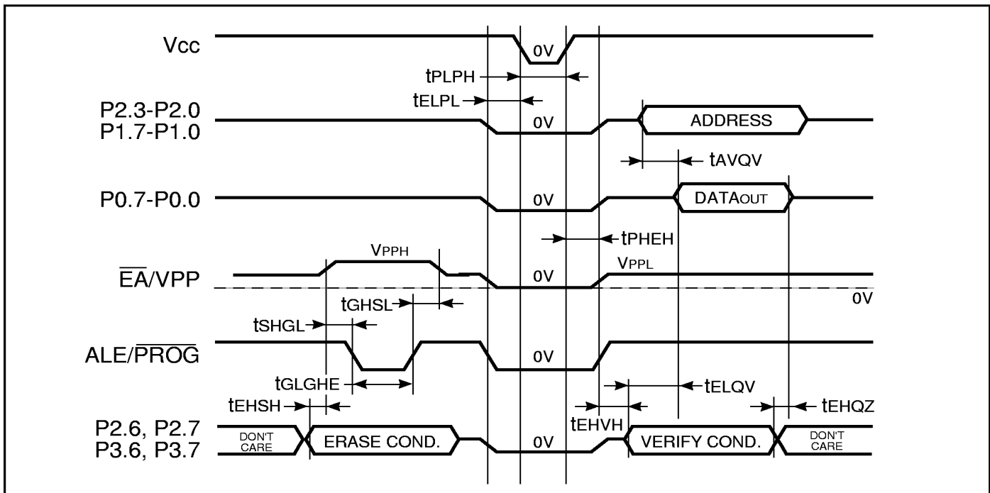
Figure 30. Flash Memory Erase Timing Waveform
