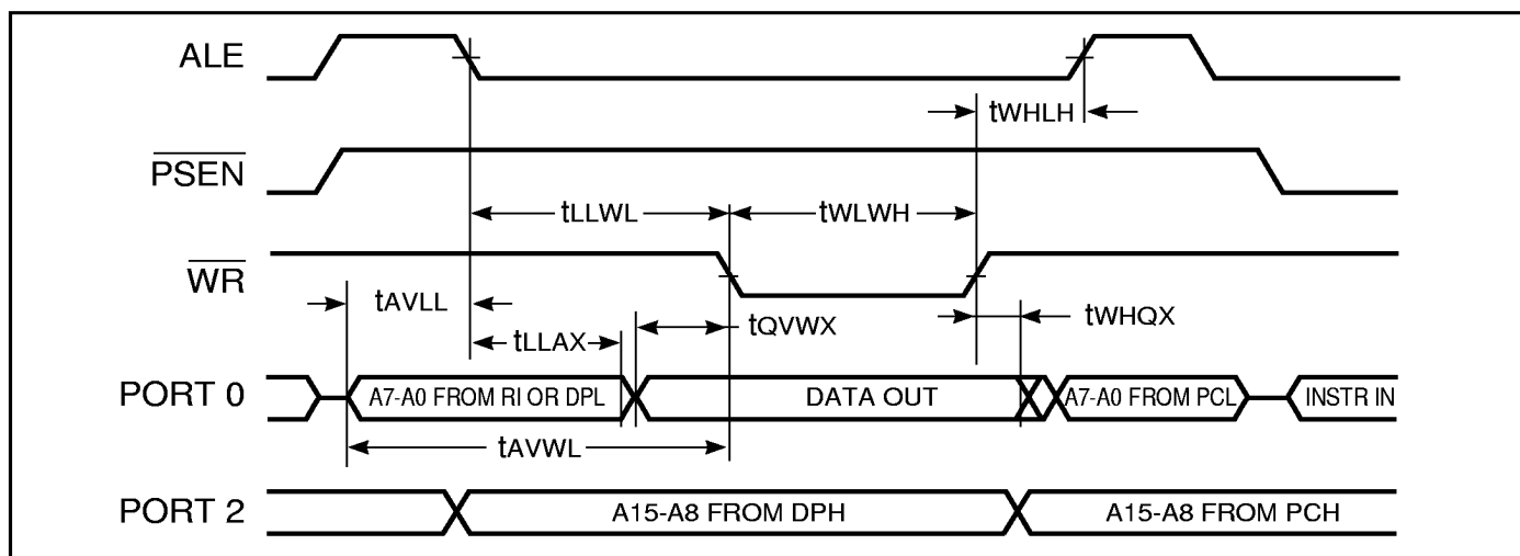
Figure 37. External Data Memory Write Cycle
