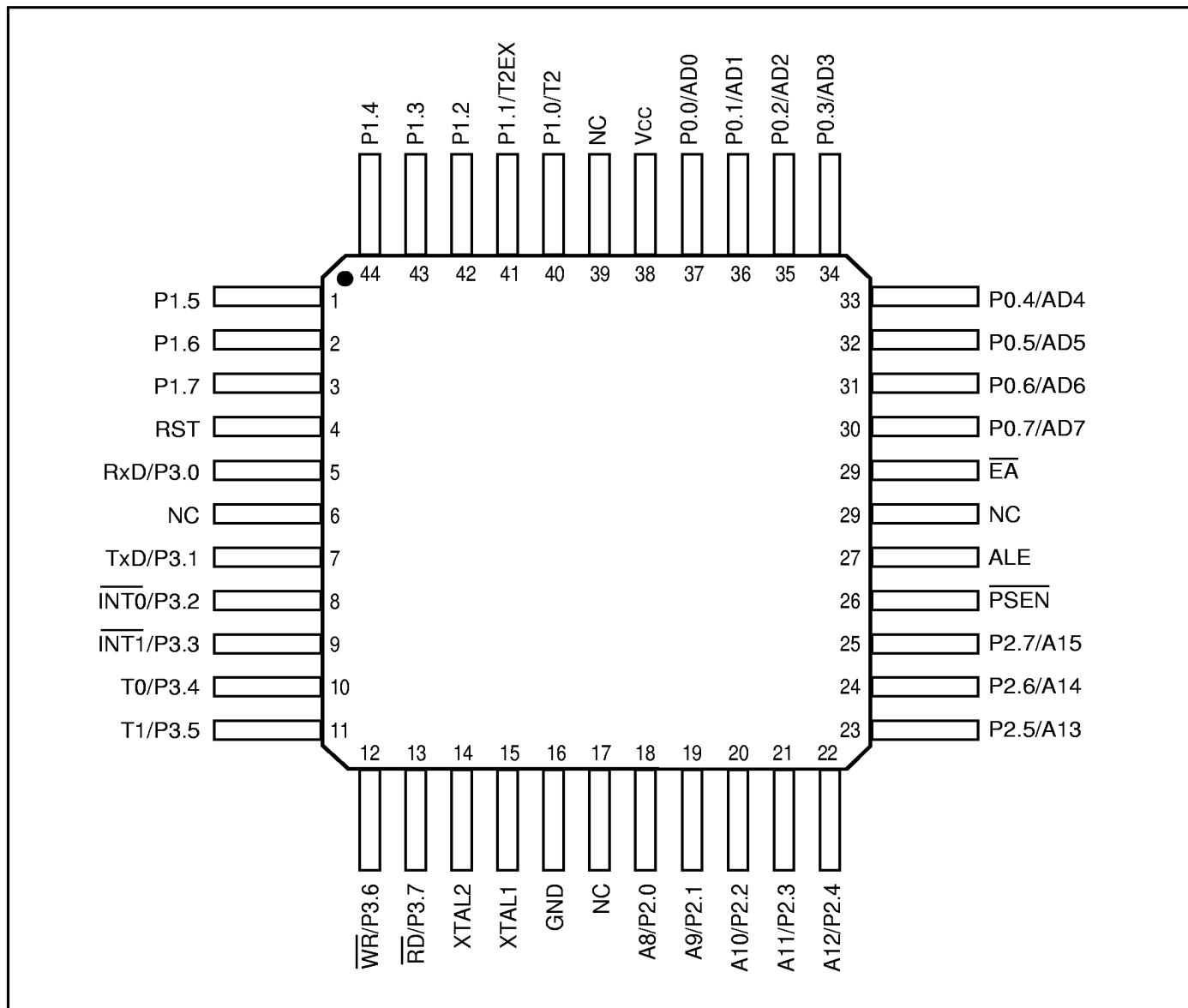
Figure 3. IS89C52 Pin Configuration: 44-pin PQFP
