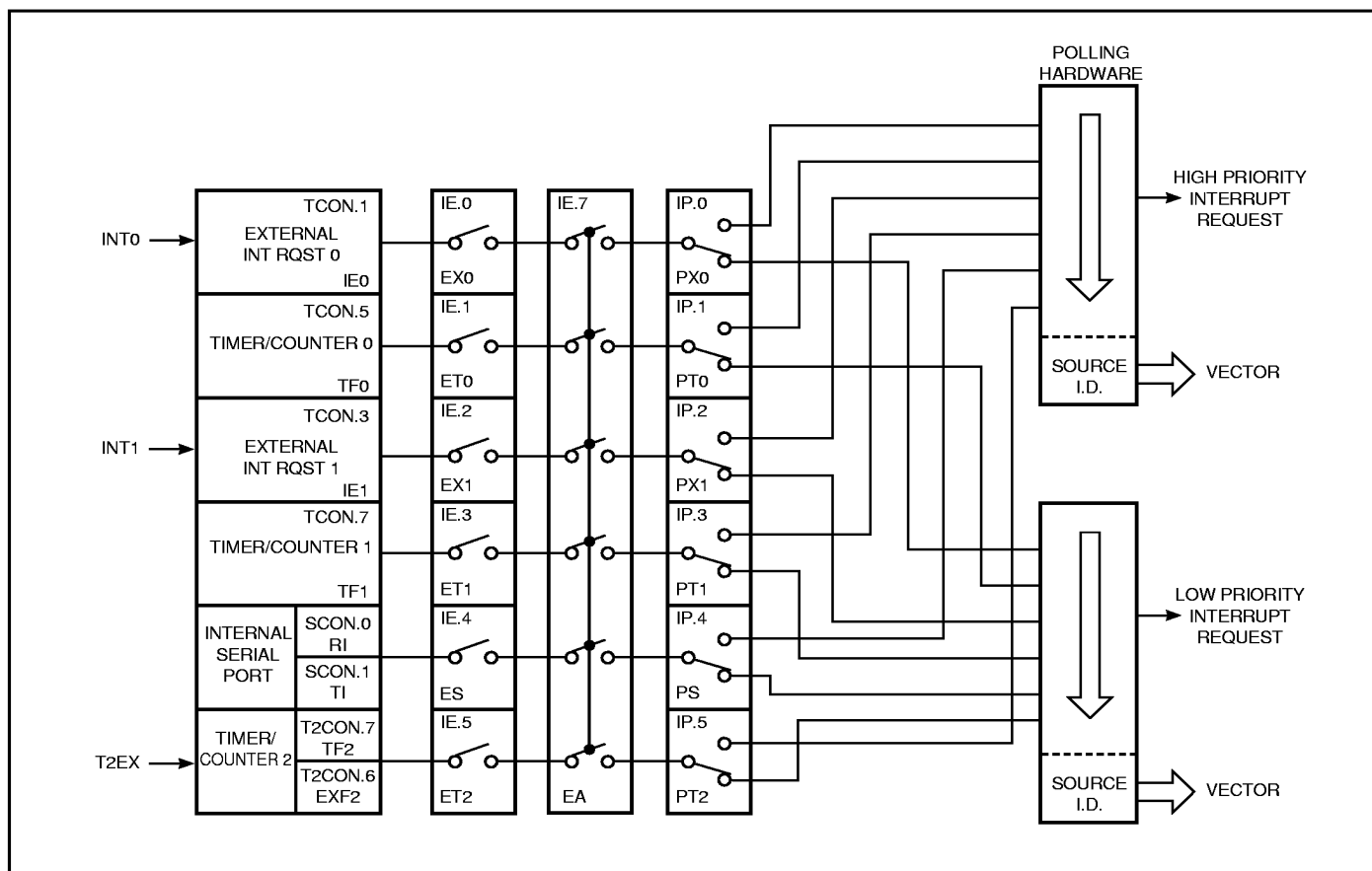
Figure 19. Interrupt System
