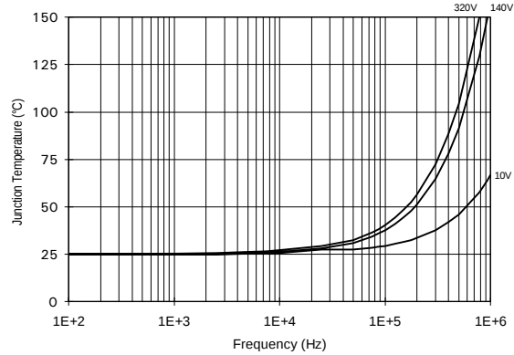
Figure 33. IR2112S T_J vs. Frequency (IRFBC30) R_{GATE} = 22\Omega , V_{CC} = 15V
