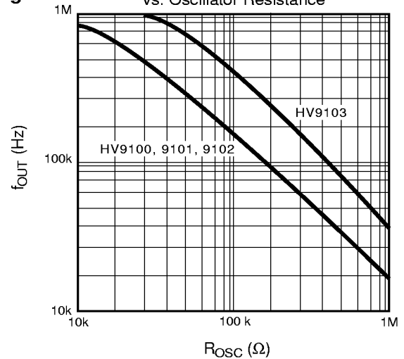
Fig. 4 Output Switching Frequency vs. Oscillator Resistance
