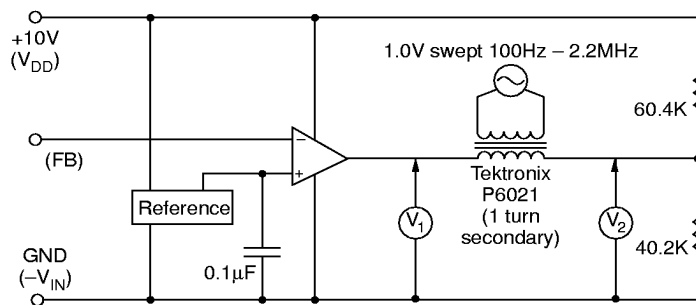
Error Amp Z_{OUT}
