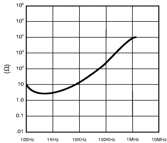
Fig. 2 Error Amplifier Output Impedance ( Z_0 )
