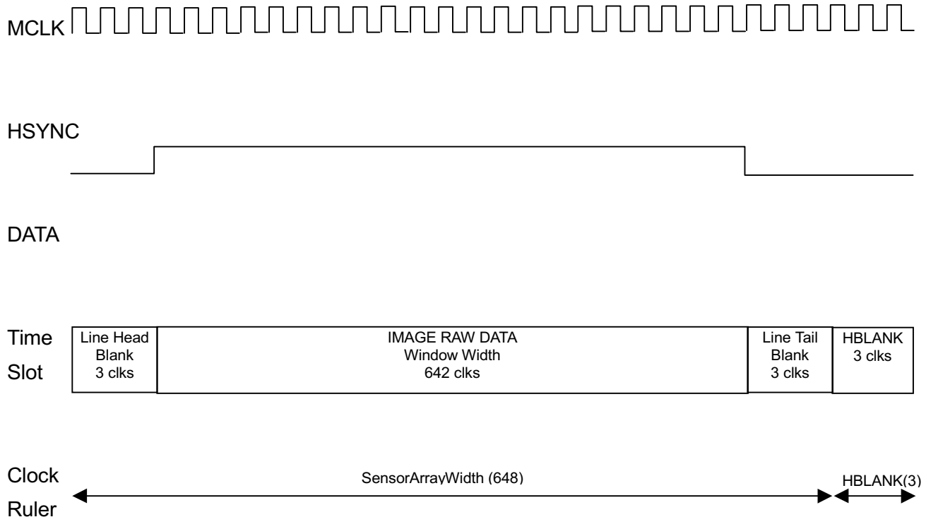
Fig.2 Even Line Data Timing
