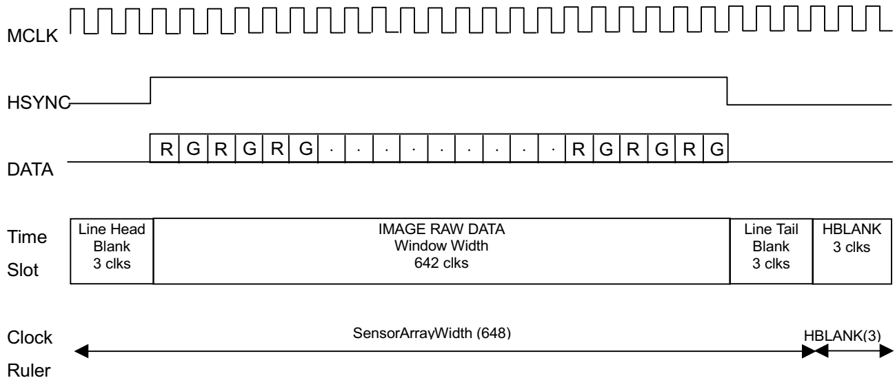
Fig.6 Even Line Data Timing
