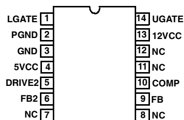
ISL6529 (SOIC) TOP VIEW
