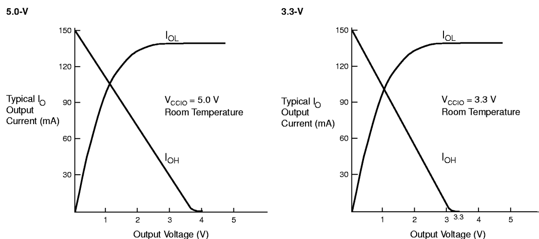
Figure 13. Output Drive Characteristics of MAX 9000 Devices
