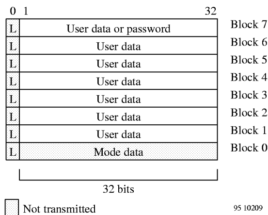
Figure 6. Memory map
