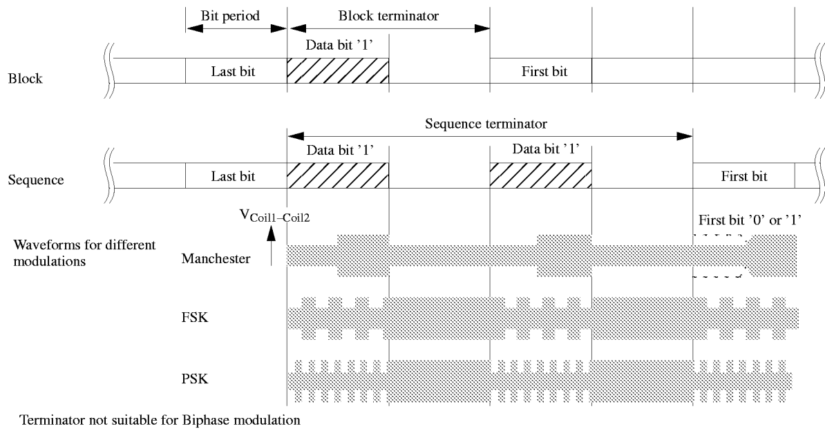
Figure 10. Terminators
