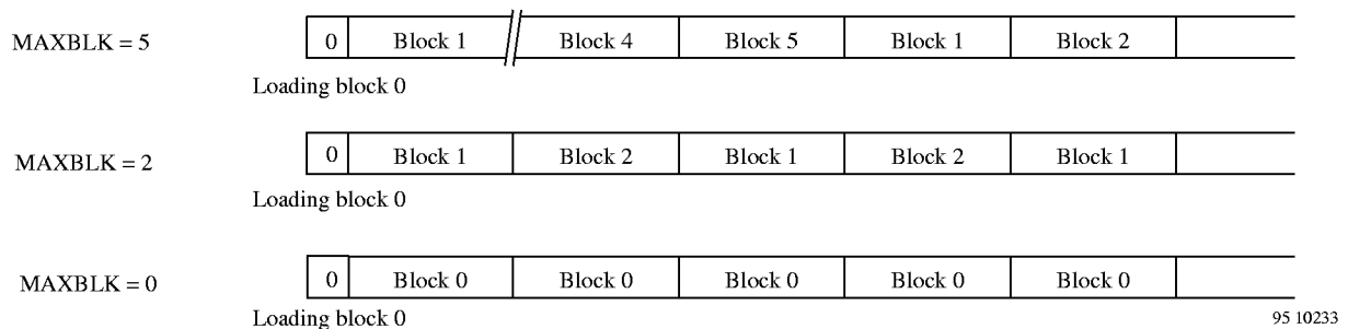
Figure 12. MAXBLK examples
