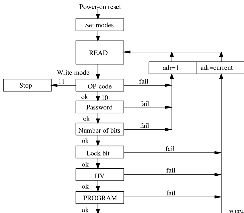
Figure 21. Functional diagram of the e5550
