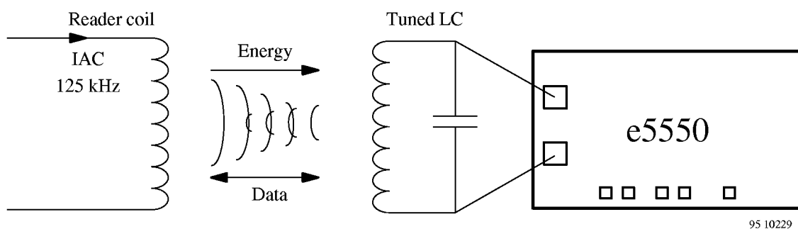
Figure 8. Application circuit
