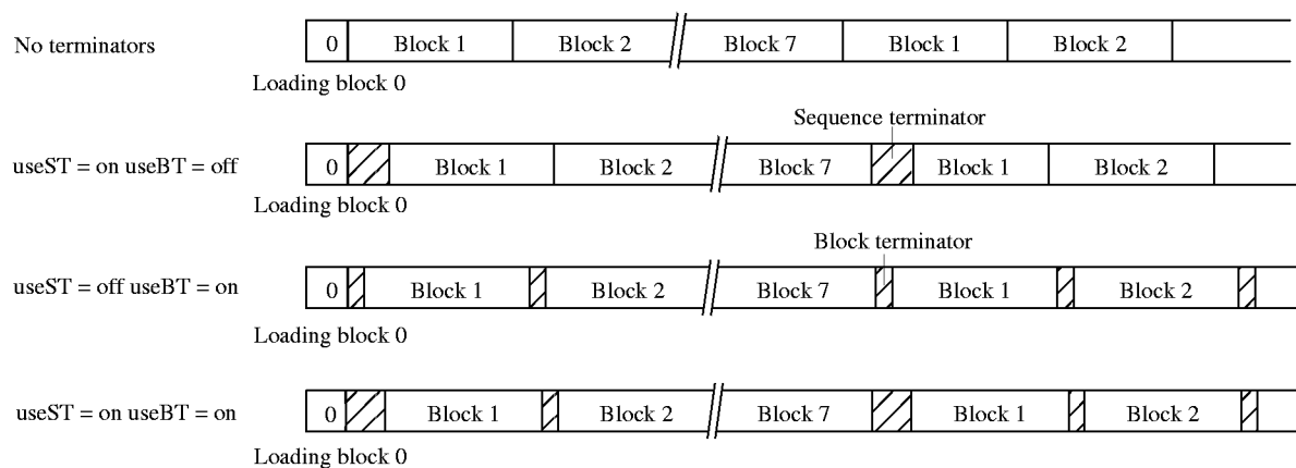
Figure 11. Read data streams and terminators
