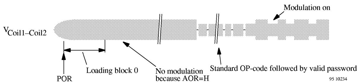
Figure 13. Answer-on-request mode
