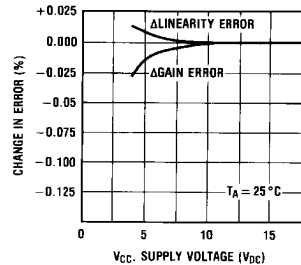
Gain and Linearity Error Variation vs. Supply Voltage
