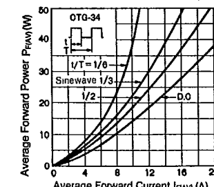
PF(AV)-IF(AV) Characteristics (CTG-34)
