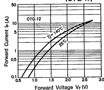
I F -V F Characteristics (CTG-12)
