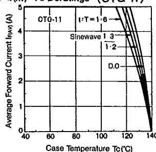
I F(AV) -T c Deratings (CTG-11)
