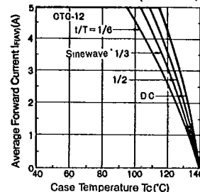
IF(AV)-Tc Deratings (CTG-12)
