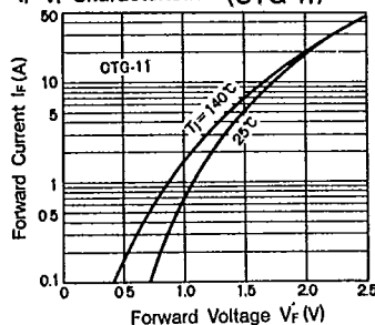
I F -V F Characteristics (CTG-11)
