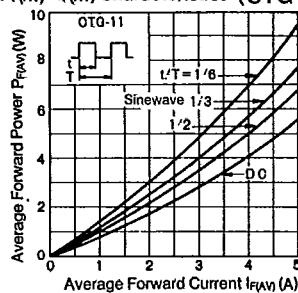
P F(AV) -I F(AV) Characteristics (CTG-11)
