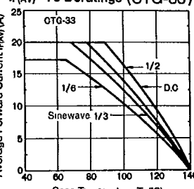
IF(AV)-Tc Deratings (CTG-33)
