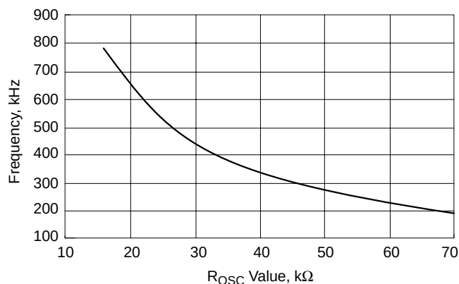
Figure 3. Oscillator Frequency
