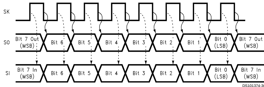
FIGURE 32. MICROWIRE/PLUS SPI Mode Interface Timing, Normal SK Mode, SK Idle Phase being Low
