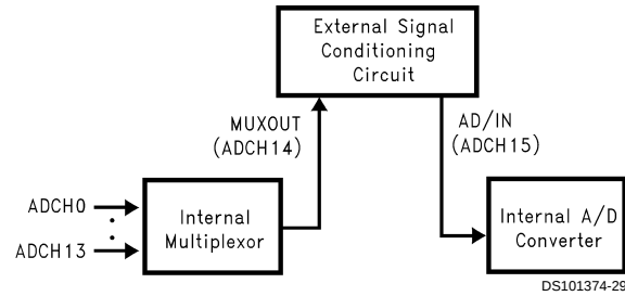
FIGURE 25. A/D with Single Ended Mux Output Feature Enabled
