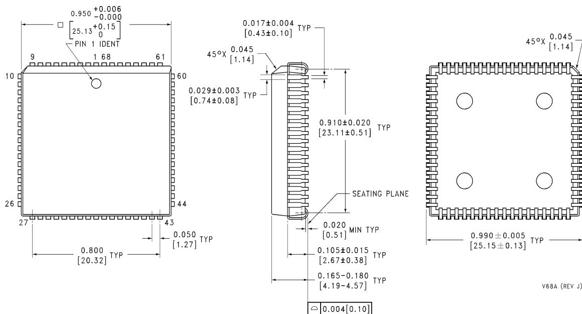
Plastic Leaded Chip Carrier (VA) Order Number COP8CBR9LVA8 or COP8CCR9LVA8 or COP8CDR9LVA8 NS Package Number V68A
