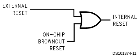
FIGURE 8. Reset Logic
