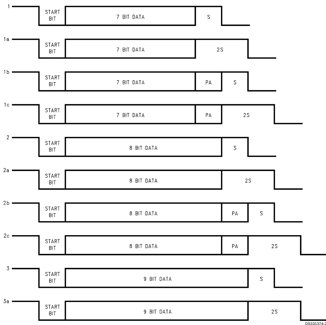
FIGURE 22. Framing Formats
