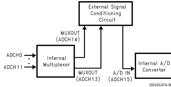
FIGURE 26. A/D with Differential Mux Output Feature Enabled
