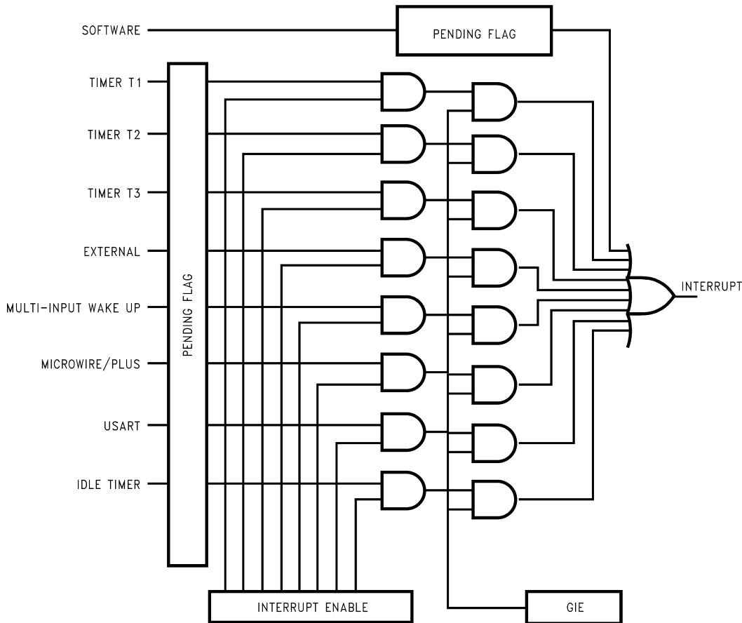
FIGURE 28. Interrupt Block Diagram
