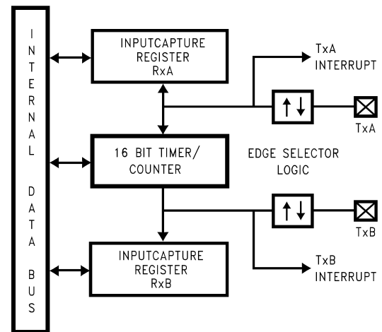
FIGURE 17. Timer in Input Capture Mode
