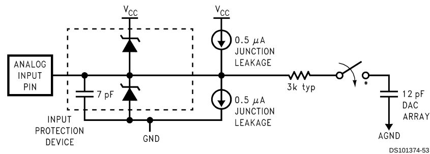
FIGURE 27. A/D Pin Model (Single Ended Mode)
