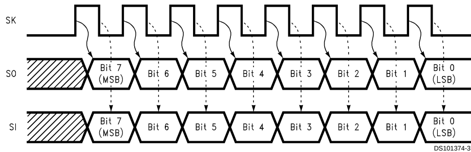
FIGURE 33. MICROWIRE/PLUS SPI Mode Interface Timing, Alternate SK Mode, SK Idle Phase being Low
