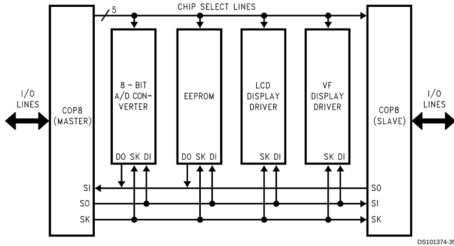
FIGURE 31. MICROWIRE/PLUS Application
