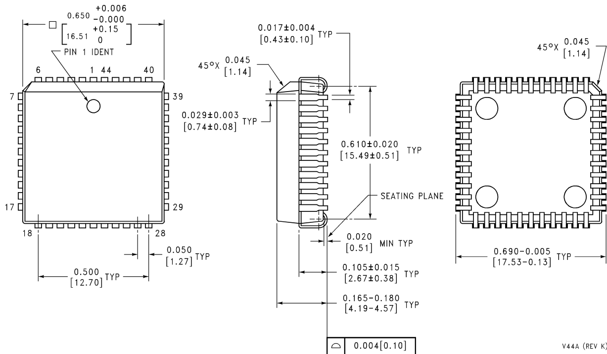
Plastic Leaded Chip Carrier (VA) Order Number COP8CBR9HVA8 or COP8CCR9HVA8 or COP8CDR9HVA8 NS Package Number V44A
