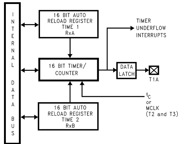
FIGURE 15. Timer in PWM Mode
