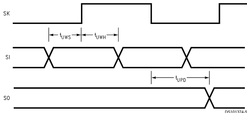
FIGURE 2. MICROWIRE/PLUS Timing
