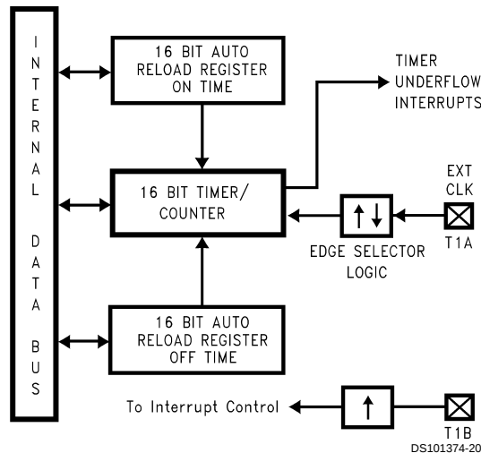
FIGURE 16. Timer in External Event Counter Mode
