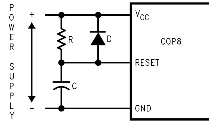
FIGURE 9. Reset Circuit Using External Reset
