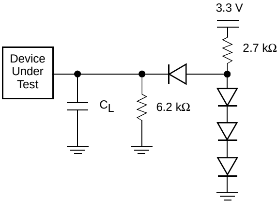
Figure 10. Test Setup
