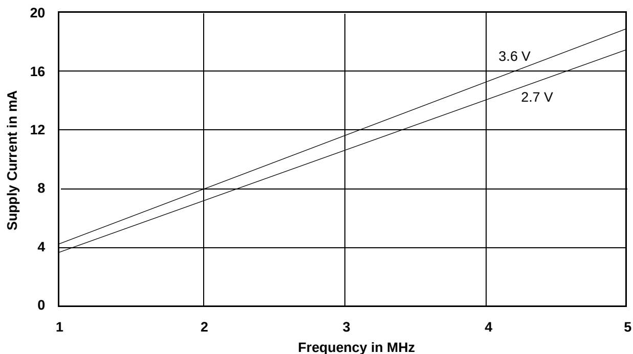
Figure 9. Typical I_{CC1} vs. Frequency
