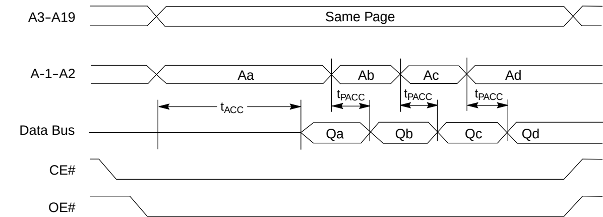
Figure 13. Page Read Timings
