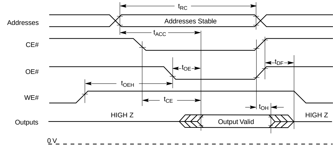
Figure 12. Conventional Read Operations Timings
