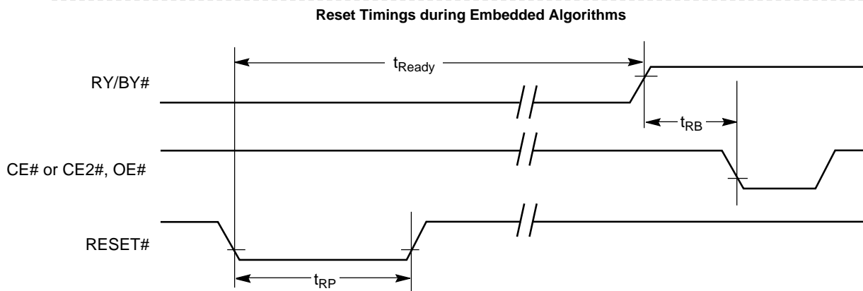
Figure 14. Reset Timings
