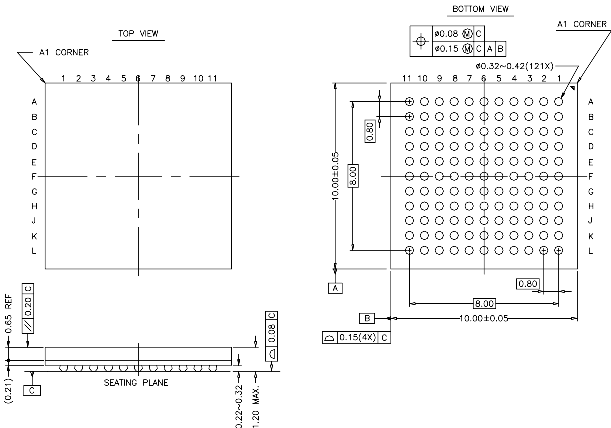
Figure 4. AT91FR4042 Package
