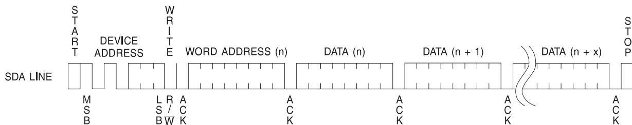
Figure 4. Page Write
