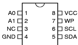
8-Pin PDIP
