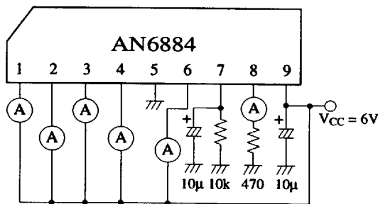
Test Circuit 3 (I (SINK) 1, 2, 3, 4, 6)
