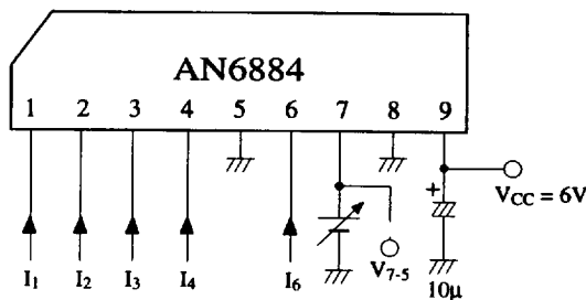
Test Circuit 5 (GD 1-5 )
