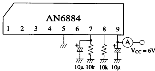
Test Circuit 1 (I CC )
