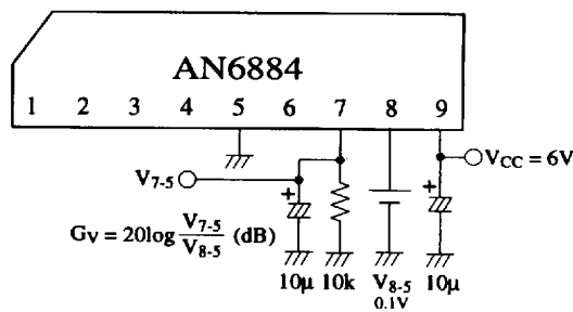
Test Circuit 4 (G V )
