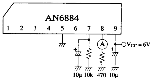
Test Circuit 2 (I Bias8 )
