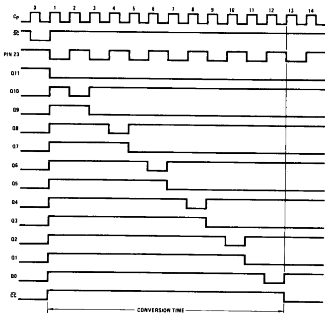
FIGURE 1d. Timing Diagram for V_{IN} = -3.4125V (0101010101)
