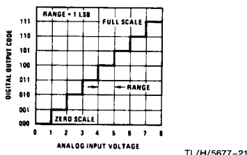
FIGURE 10. Quantization Uncertainty of a Perfect 3-Bit A/D
