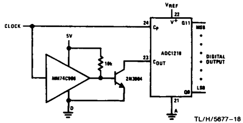
FIGURE 9. Conversion at 26 μs
