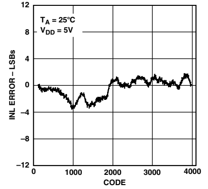
Figure 7. AD5340 Typical INL Plot
