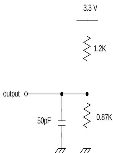
AC TEST LOAD (A)
