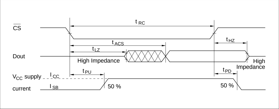
Read Timing Waveform (2) *1, *3
