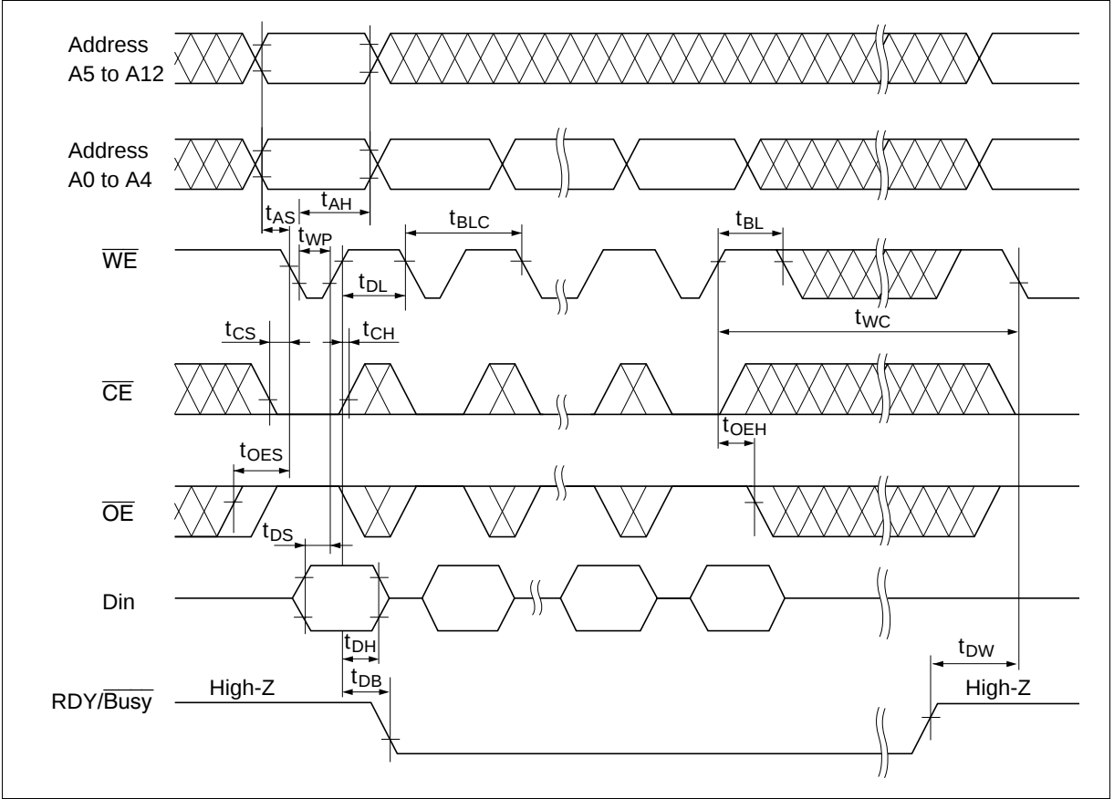
Page Write Timing Waveform (1) ( \overline{\text{WE}} Controlled)
