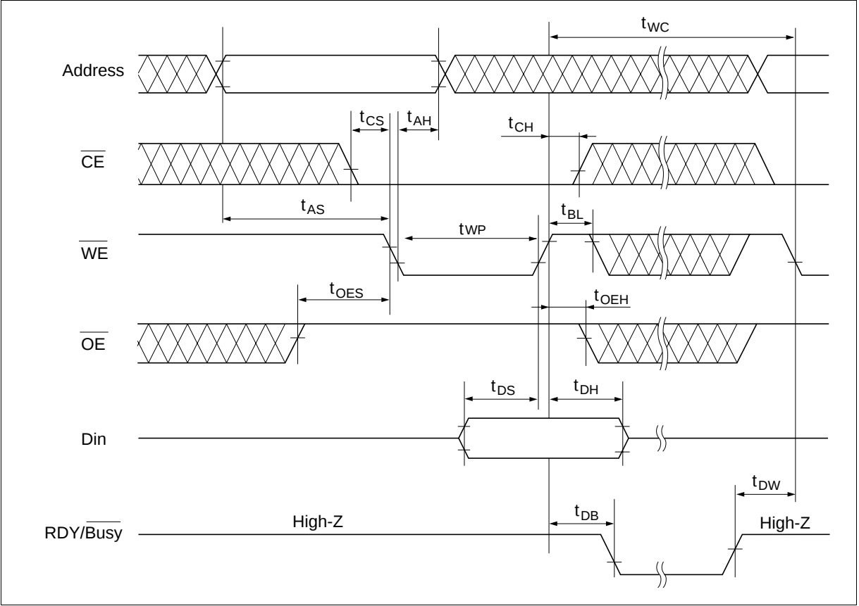
Byte Write Timing Waveform (1) ( \overline{\text{WE}} Controlled)
