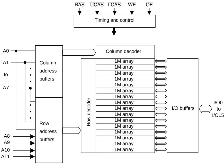
Block Diagram (HM51W18160 Series)
