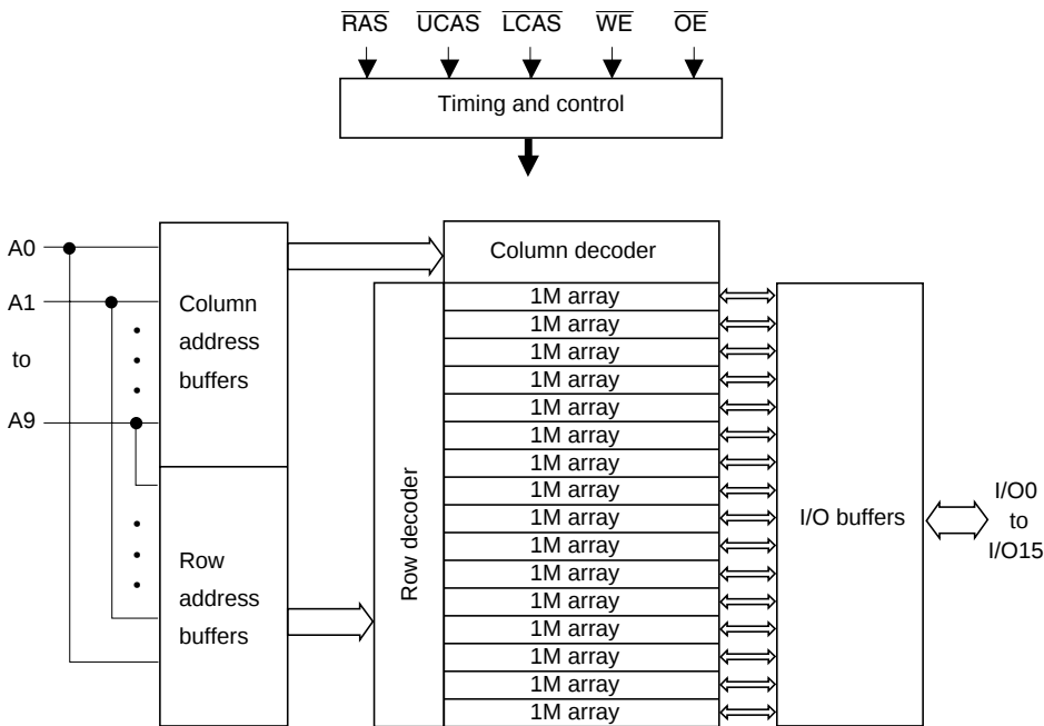
Block Diagram (HM51W18160 Series)
