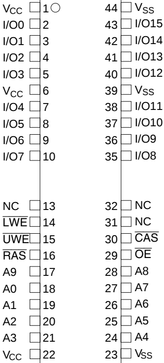
(Top view)
