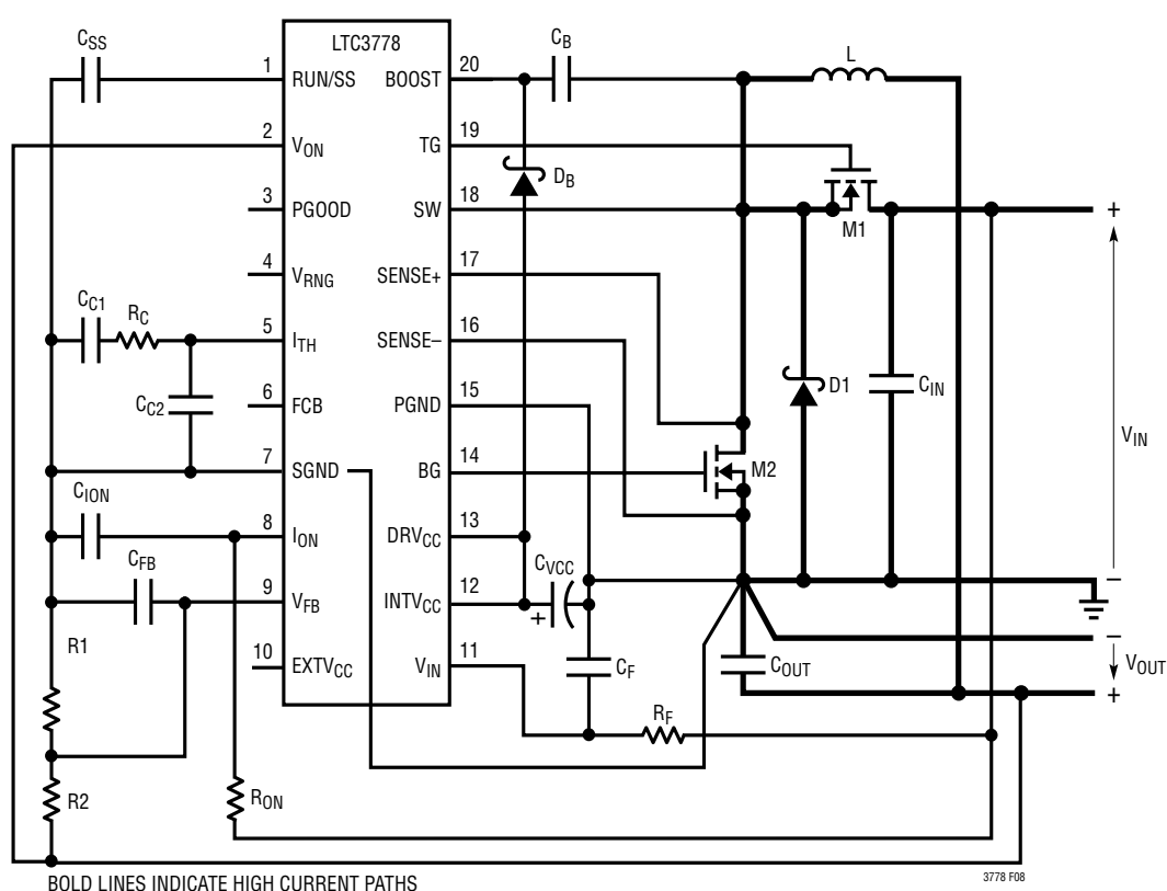
Figure 8. LTC3778 Layout Diagram
