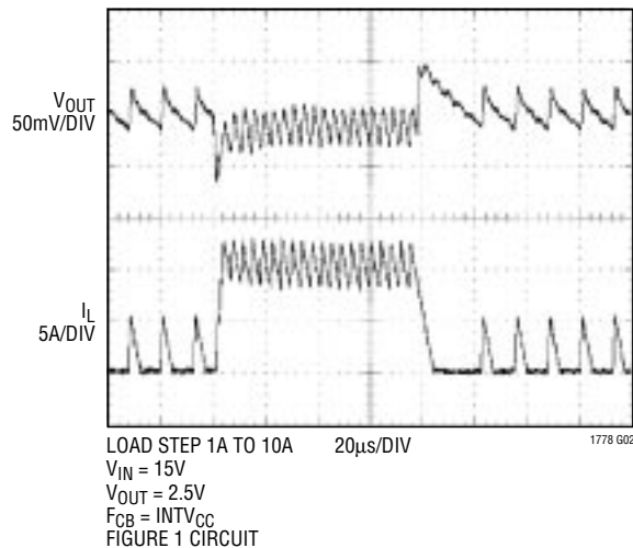
Transient Response (Discontinuous Mode)
