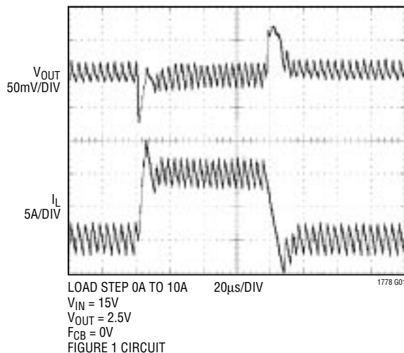
Transient Response
