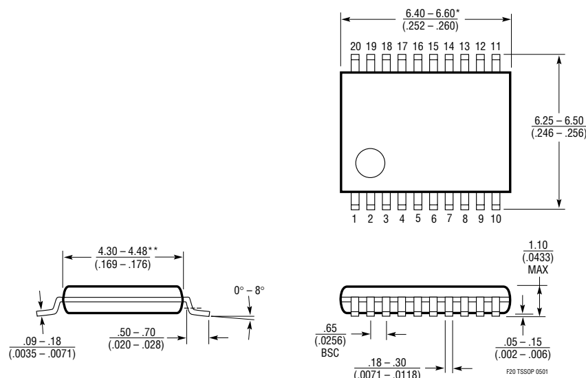
F Package 20-Lead Plastic TSSOP (4.4mm) (Reference LTC DWG # 05-08-1650)
