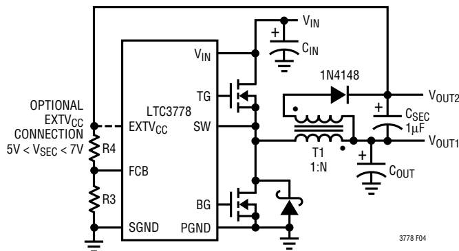
Figure 4. Secondary Output Loop and EXTV CC Connection
