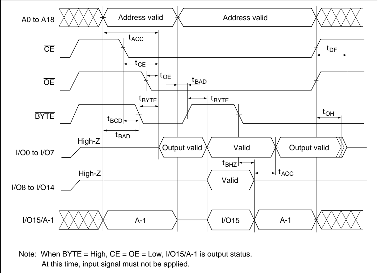
Read Timing Waveform (Byte Mode, Word Mode Switch)
