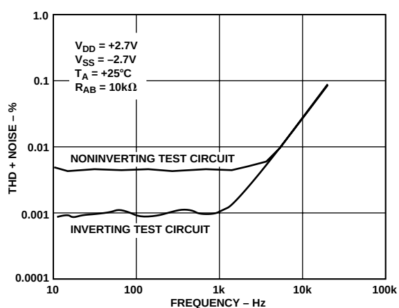
Figure 15. Total Harmonic Distortion Plus Noise vs. Frequency
