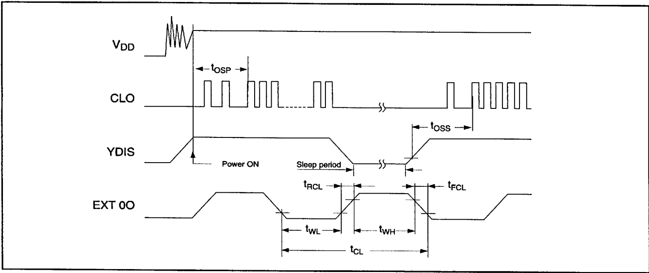
Figure 37. Oscillator timing
