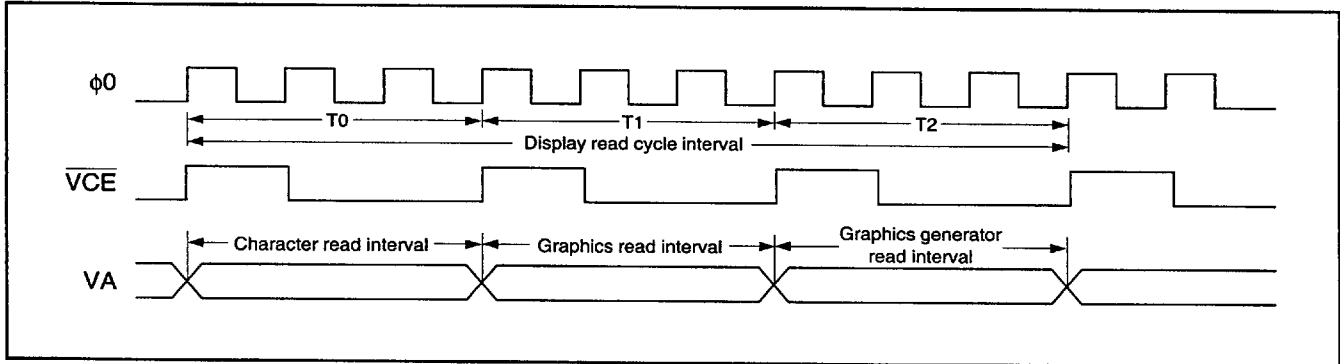
Figure 52. Display memory basic read cycle
