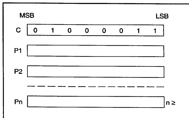
Figure 31. MREAD parameters
